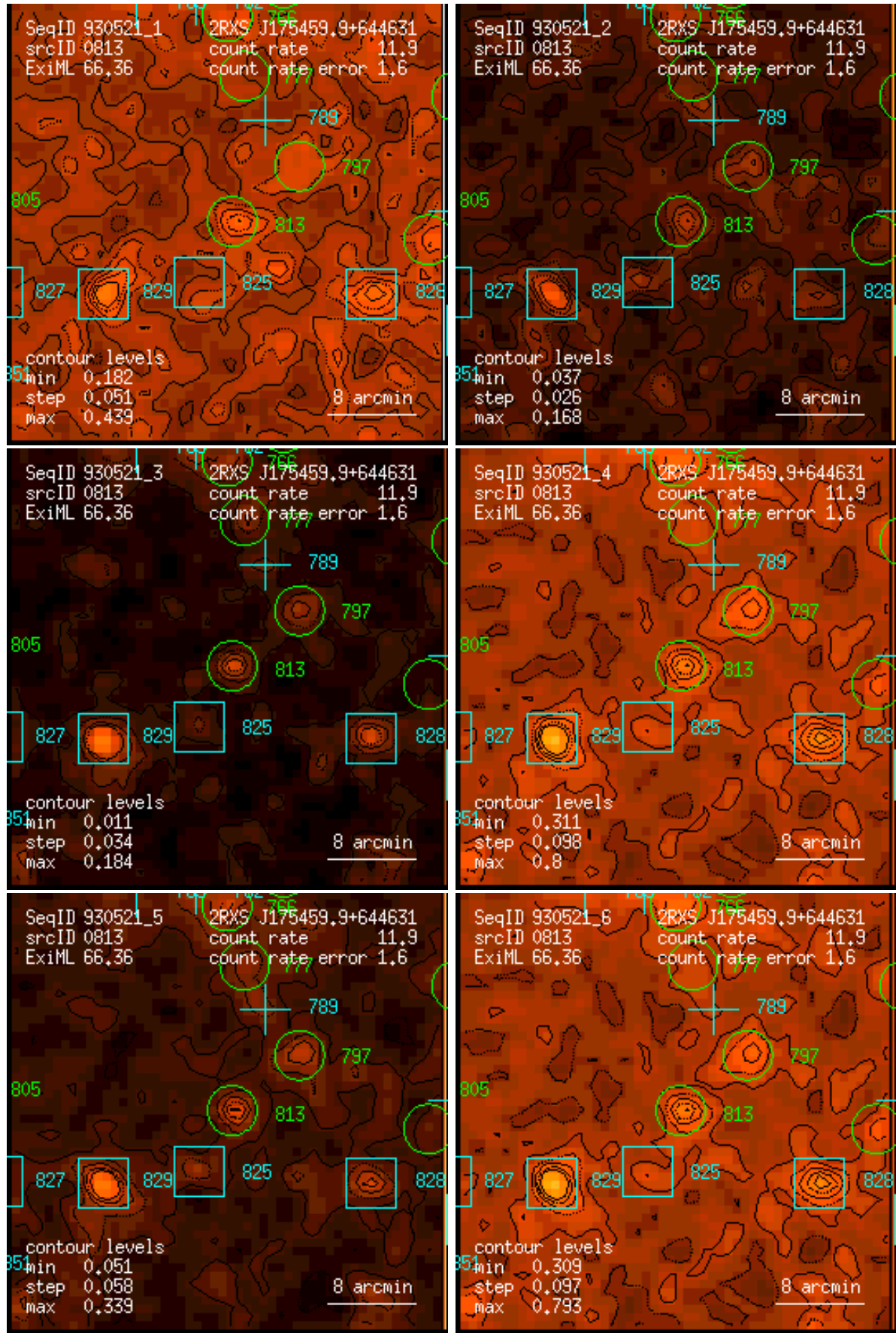
Figure 813: RASS 930521: detection 0813: band rate images, Gaussian filter: (1) PSPC channels 11 – 41, (2) 52 – 90, (3) 91 – 201, (4) 11 – 235, (5) 52 – 201, (6) 11 – 201. Broad band rates in counts/ks. Band rate contour levels in counts/ks/arcmin 2 .
