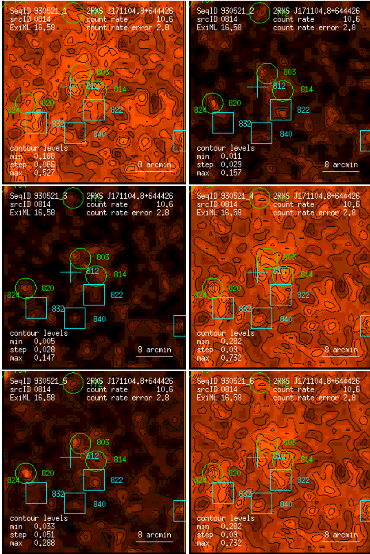
Figure 814: RASS 930521: detection 0814: band rate images, Gaussian filter: (1) PSPC channels 11 – 41, (2) 52 – 90, (3) 91 – 201, (4) 11 – 235, (5) 52 – 201, (6) 11 – 201. Broad band rates in counts/ks. Band rate contour levels in counts/ks/arcmin 2 .
