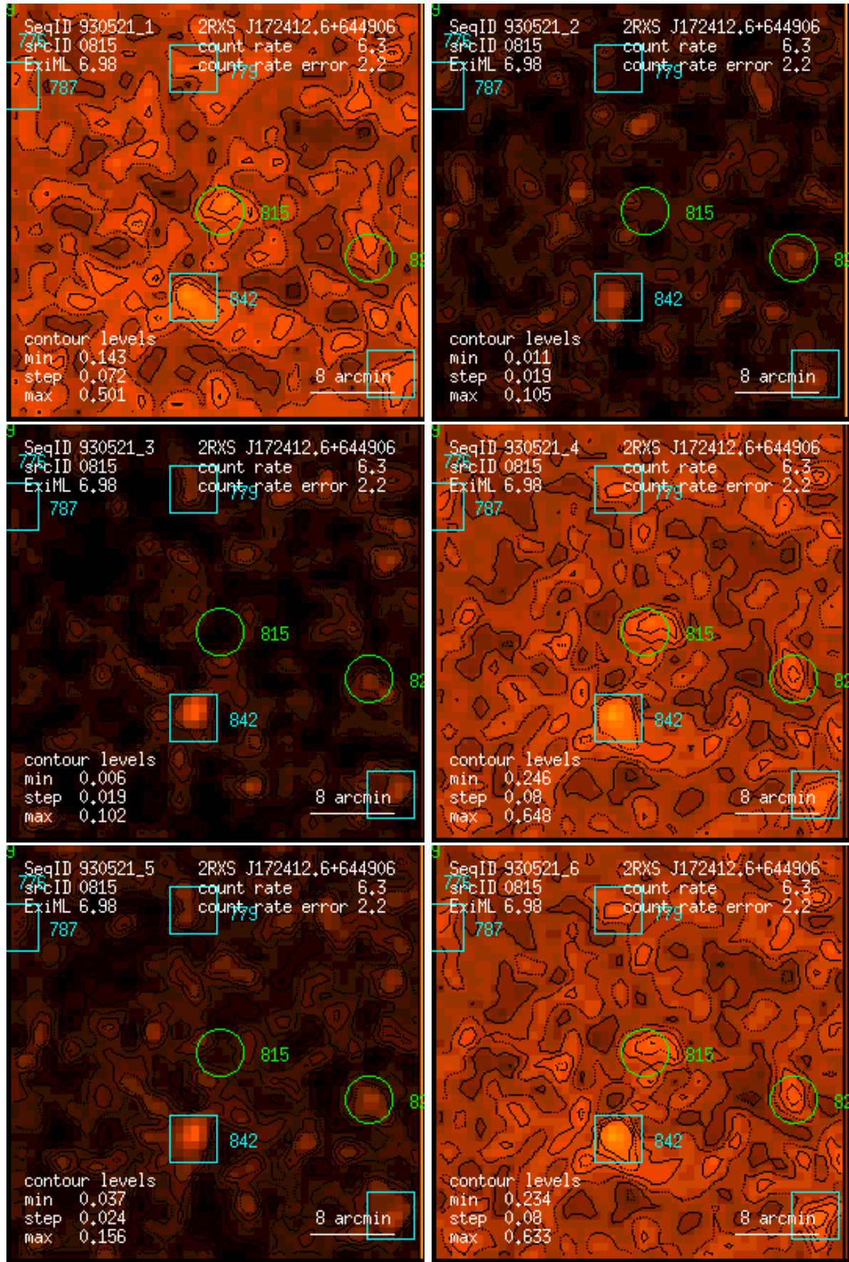
Figure 815: RASS 930521: detection 0815: band rate images, Gaussian filter: (1) PSPC channels 11 – 41, (2) 52 – 90, (3) 91 – 201, (4) 11 – 235, (5) 52 – 201, (6) 11 – 201. Broad band rates in counts/ks. Band rate contour levels in counts/ks/arcmin 2 .
