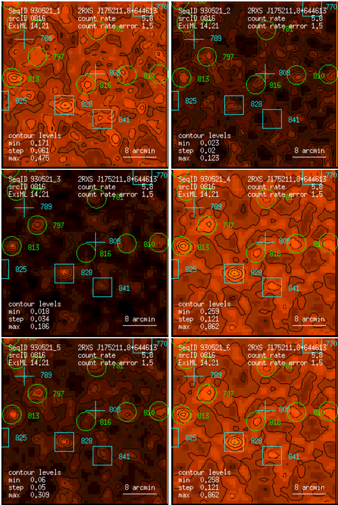
Figure 816: RASS 930521: detection 0816: band rate images, Gaussian filter: (1) PSPC channels 11 – 41, (2) 52 – 90, (3) 91 – 201, (4) 11 – 235, (5) 52 – 201, (6) 11 – 201. Broad band rates in counts/ks. Band rate contour levels in counts/ks/arcmin 2 .
