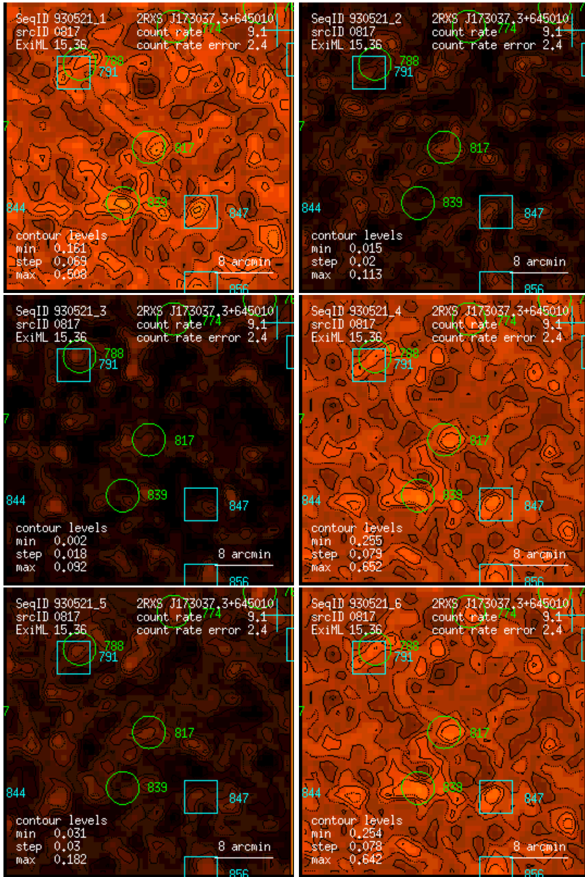
Figure 817: RASS 930521: detection 0817: band rate images, Gaussian filter: (1) PSPC channels 11 – 41, (2) 52 – 90, (3) 91 – 201, (4) 11 – 235, (5) 52 – 201, (6) 11 – 201. Broad band rates in counts/ks. Band rate contour levels in counts/ks/arcmin 2 .
