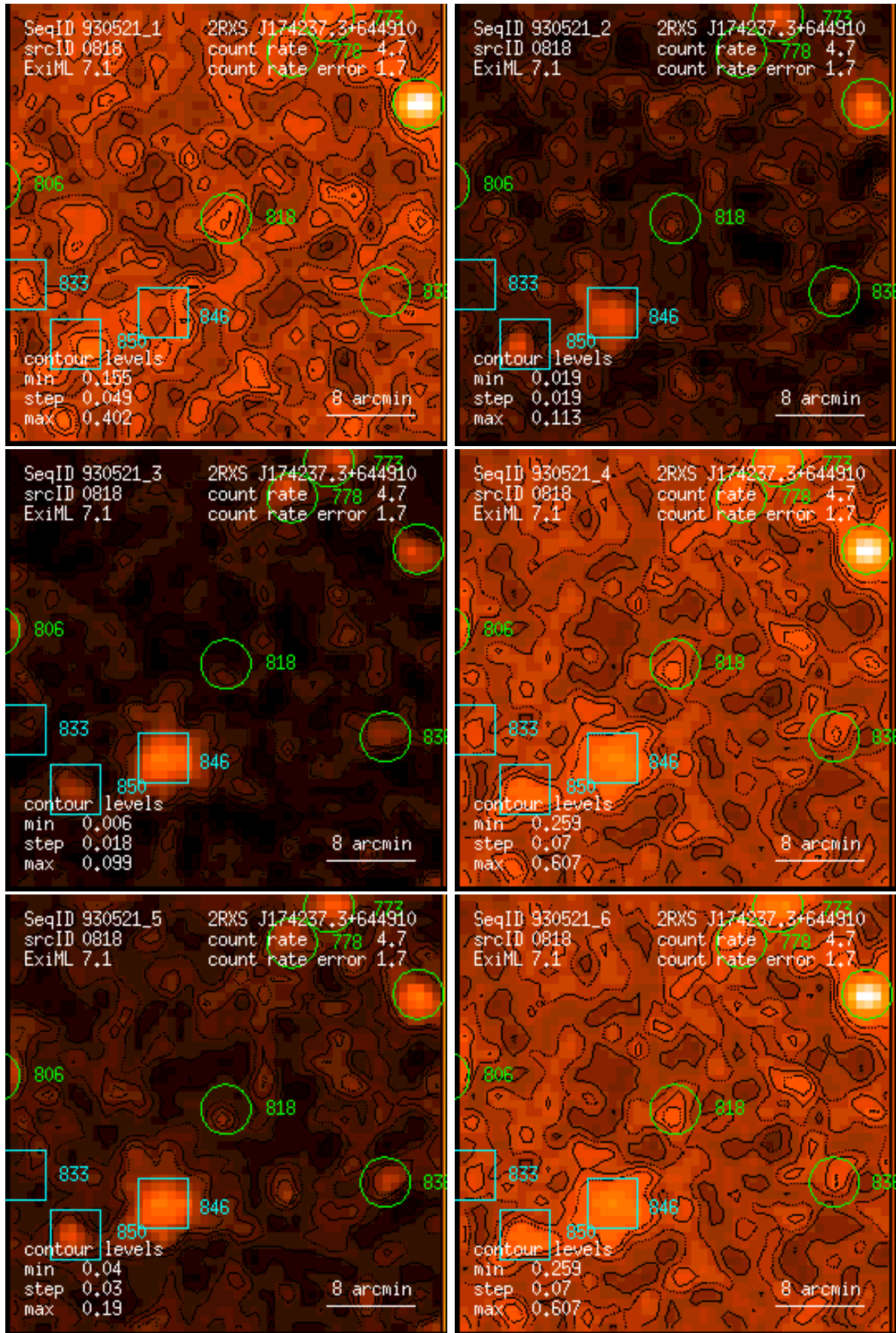
Figure 818: RASS 930521: detection 0818: band rate images, Gaussian filter: (1) PSPC channels 11 – 41, (2) 52 – 90, (3) 91 – 201, (4) 11 – 235, (5) 52 – 201, (6) 11 – 201. Broad band rates in counts/ks. Band rate contour levels in counts/ks/arcmin 2 .
