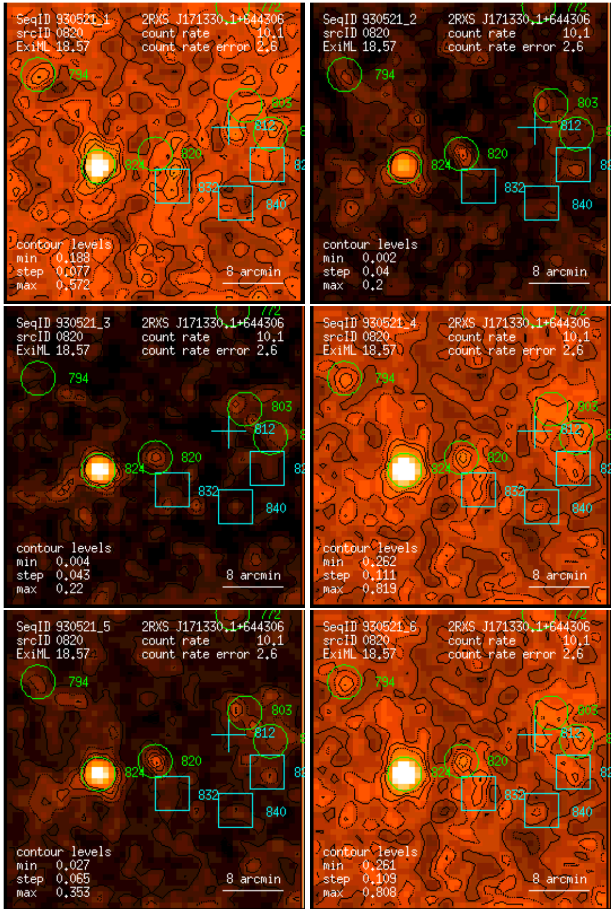
Figure 820: RASS 930521: detection 0820: band rate images, Gaussian filter: (1) PSPC channels 11 – 41, (2) 52 – 90, (3) 91 – 201, (4) 11 – 235, (5) 52 – 201, (6) 11 – 201. Broad band rates in counts/ks. Band rate contour levels in counts/ks/arcmin 2 .
