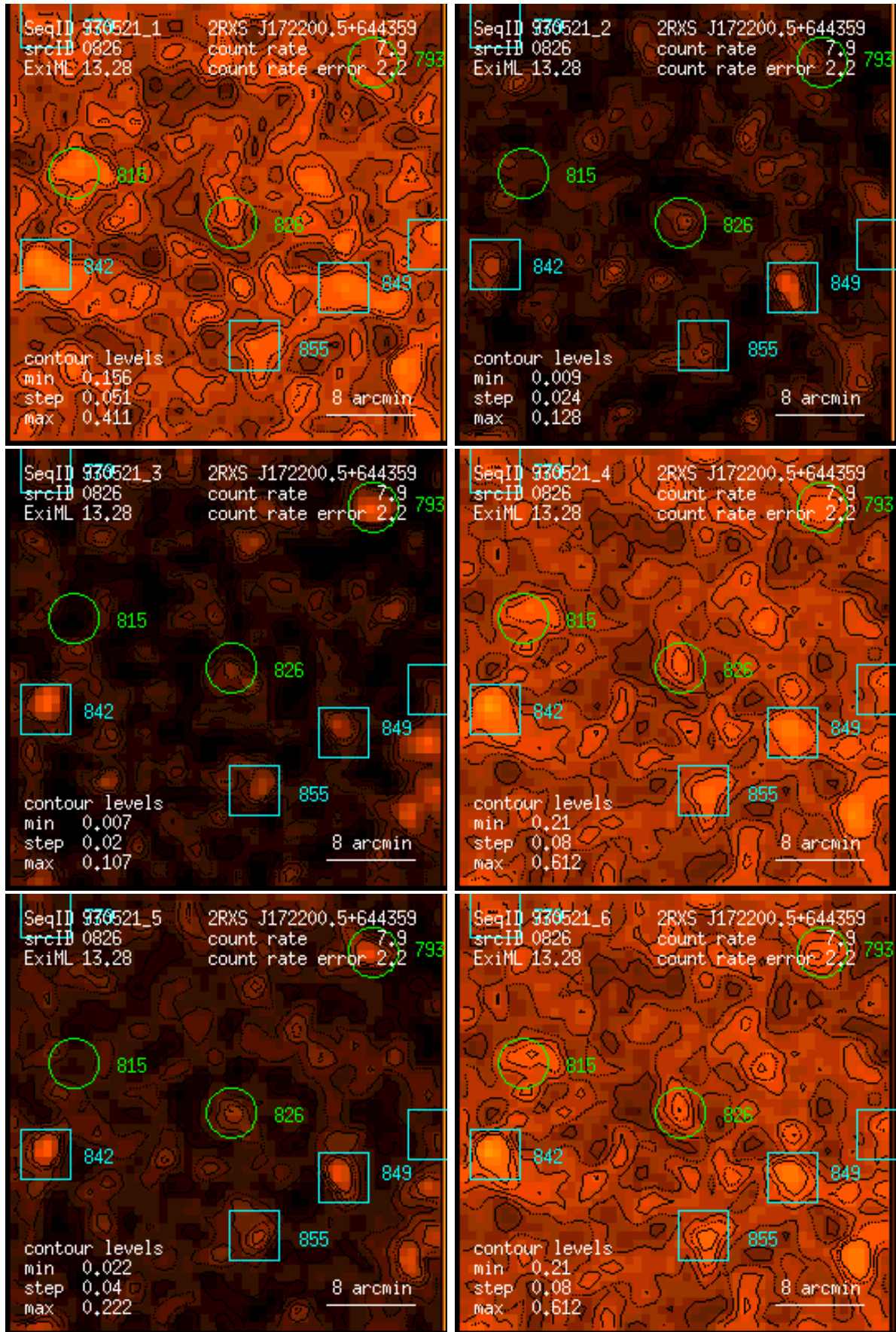
Figure 826: RASS 930521: detection 0826: band rate images, Gaussian filter: (1) PSPC channels 11 – 41, (2) 52 – 90, (3) 91 – 201, (4) 11 – 235, (5) 52 – 201, (6) 11 – 201. Broad band rates in counts/ks. Band rate contour levels in counts/ks/arcmin 2 .
