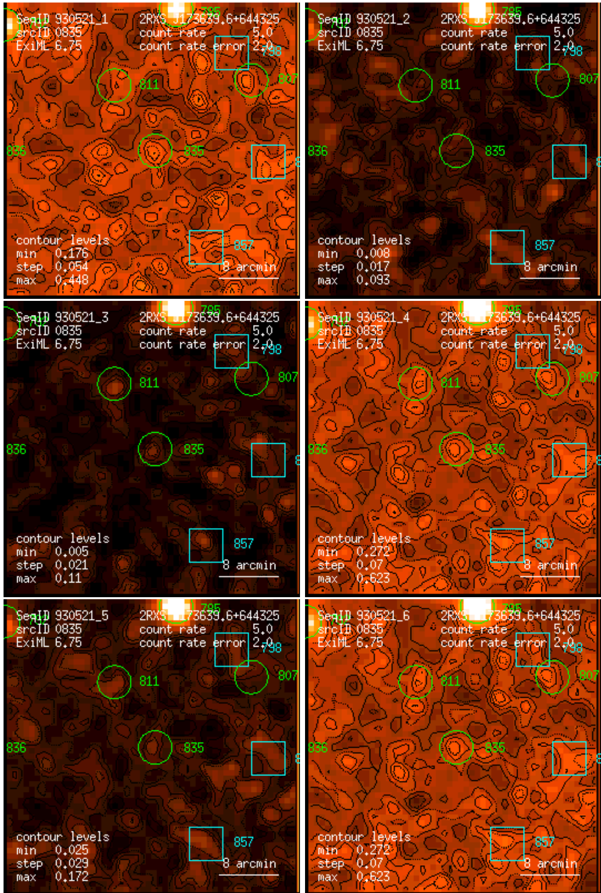
Figure 835: RASS 930521: detection 0835: band rate images, Gaussian filter: (1) PSPC channels 11 – 41, (2) 52 – 90, (3) 91 – 201, (4) 11 – 235, (5) 52 – 201, (6) 11 – 201. Broad band rates in counts/ks. Band rate contour levels in counts/ks/arcmin 2 .
