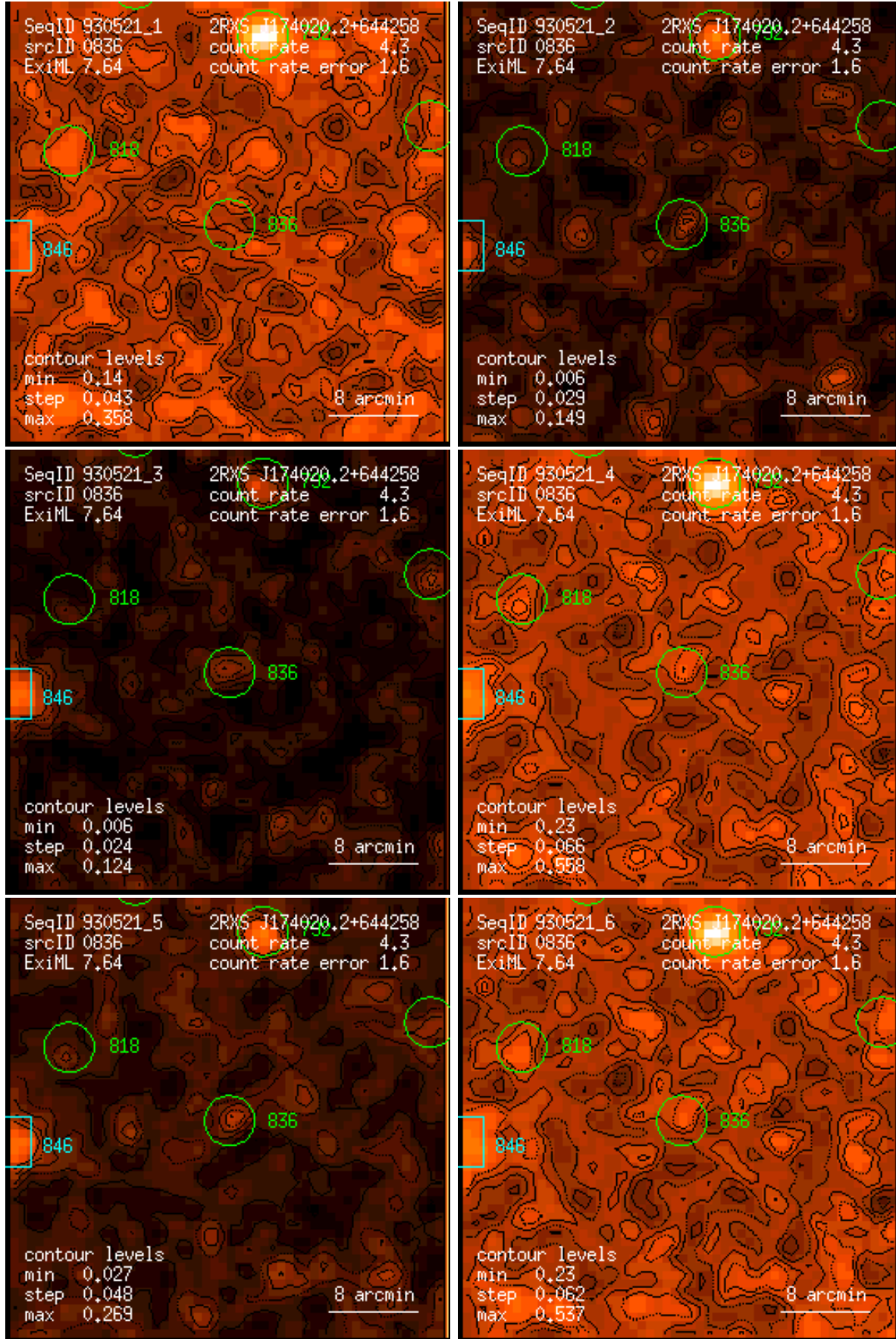
Figure 836: RASS 930521: detection 0836: band rate images, Gaussian filter: (1) PSPC channels 11 – 41, (2) 52 – 90, (3) 91 – 201, (4) 11 – 235, (5) 52 – 201, (6) 11 – 201. Broad band rates in counts/ks. Band rate contour levels in counts/ks/arcmin 2 .
