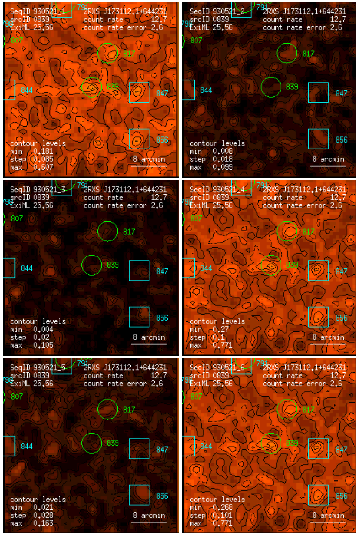
Figure 839: RASS 930521: detection 0839: band rate images, Gaussian filter: (1) PSPC channels 11 – 41, (2) 52 – 90, (3) 91 – 201, (4) 11 – 235, (5) 52 – 201, (6) 11 – 201. Broad band rates in counts/ks. Band rate contour levels in counts/ks/arcmin 2 .
