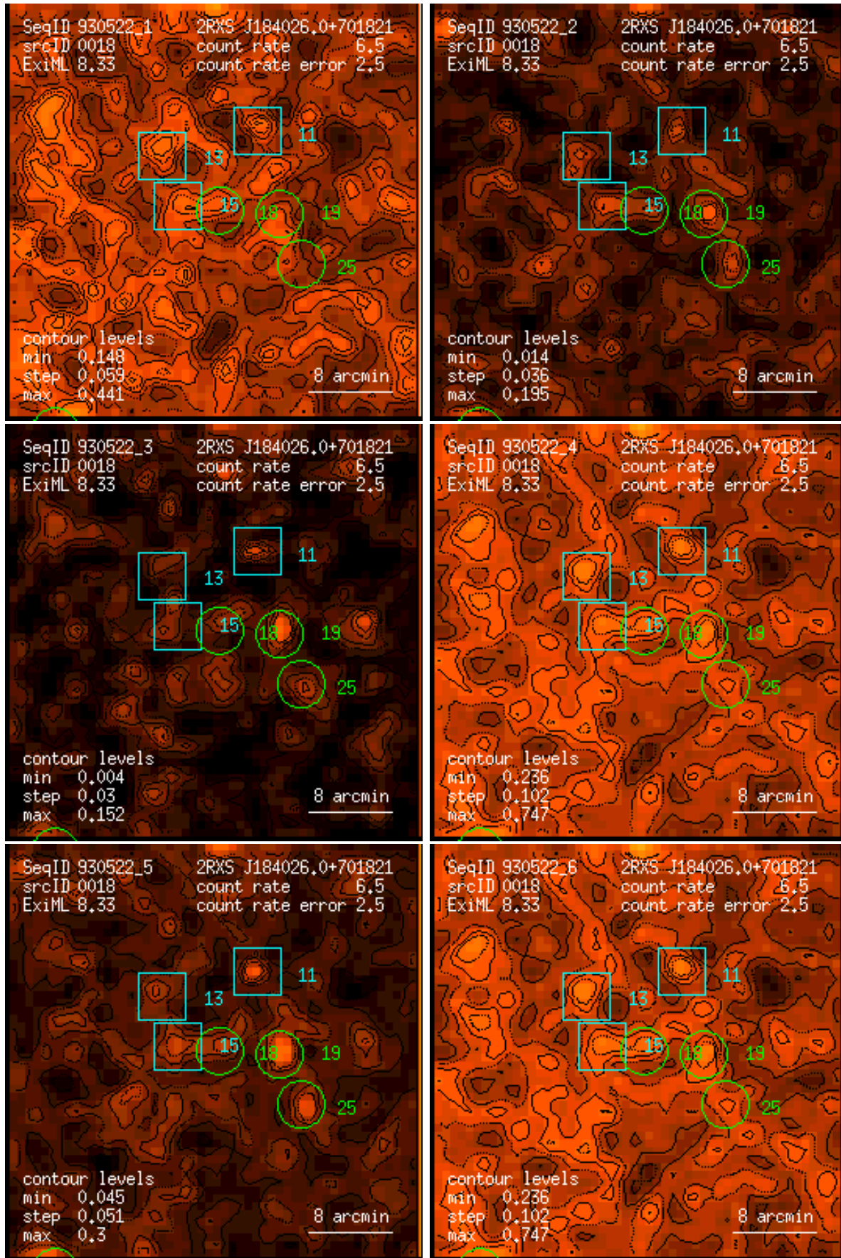
Figure 18: RASS 930522: detection 0018: band rate images, Gaussian filter: (1) PSPC channels 11 – 41, (2) 52 – 90, (3) 91 – 201, (4) 11 – 235, (5) 52 – 201, (6) 11 – 201. Broad band rates in counts/ks. Band rate contour levels in counts/ks/arcmin 2 .
