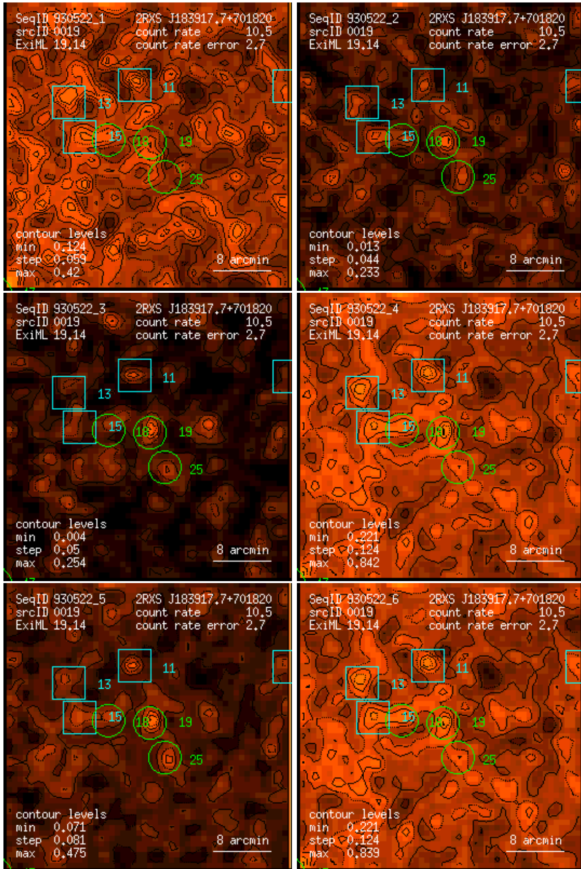
Figure 19: RASS 930522: detection 0019: band rate images, Gaussian filter: (1) PSPC channels 11 – 41, (2) 52 – 90, (3) 91 – 201, (4) 11 – 235, (5) 52 – 201, (6) 11 – 201. Broad band rates in counts/ks. Band rate contour levels in counts/ks/arcmin 2 .
