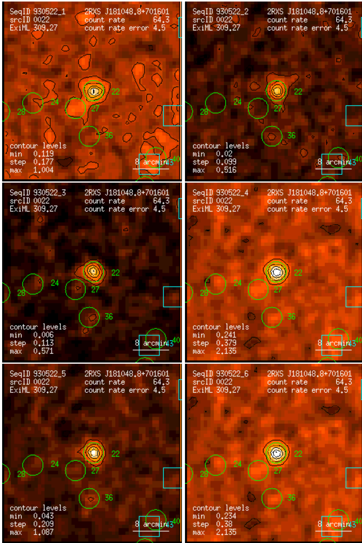
Figure 22: RASS 930522: detection 0022: band rate images, Gaussian filter: (1) PSPC channels 11 – 41, (2) 52 – 90, (3) 91 – 201, (4) 11 – 235, (5) 52 – 201, (6) 11 – 201. Broad band rates in counts/ks. Band rate contour levels in counts/ks/arcmin 2 .
