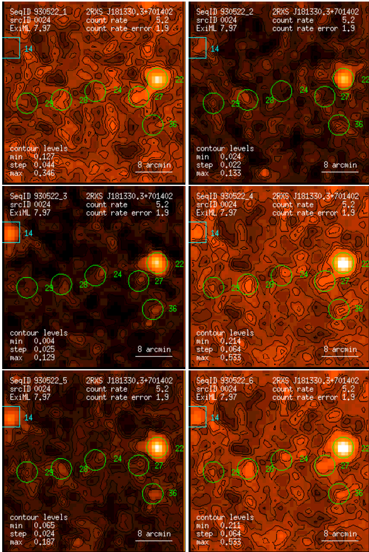
Figure 24: RASS 930522: detection 0024: band rate images, Gaussian filter: (1) PSPC channels 11 – 41, (2) 52 – 90, (3) 91 – 201, (4) 11 – 235, (5) 52 – 201, (6) 11 – 201. Broad band rates in counts/ks. Band rate contour levels in counts/ks/arcmin 2 .
