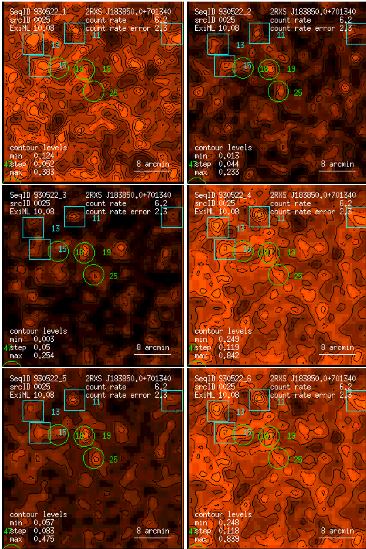
Figure 25: RASS 930522: detection 0025: band rate images, Gaussian filter: (1) PSPC channels 11 – 41, (2) 52 – 90, (3) 91 – 201, (4) 11 – 235, (5) 52 – 201, (6) 11 – 201. Broad band rates in counts/ks. Band rate contour levels in counts/ks/arcmin 2 .
