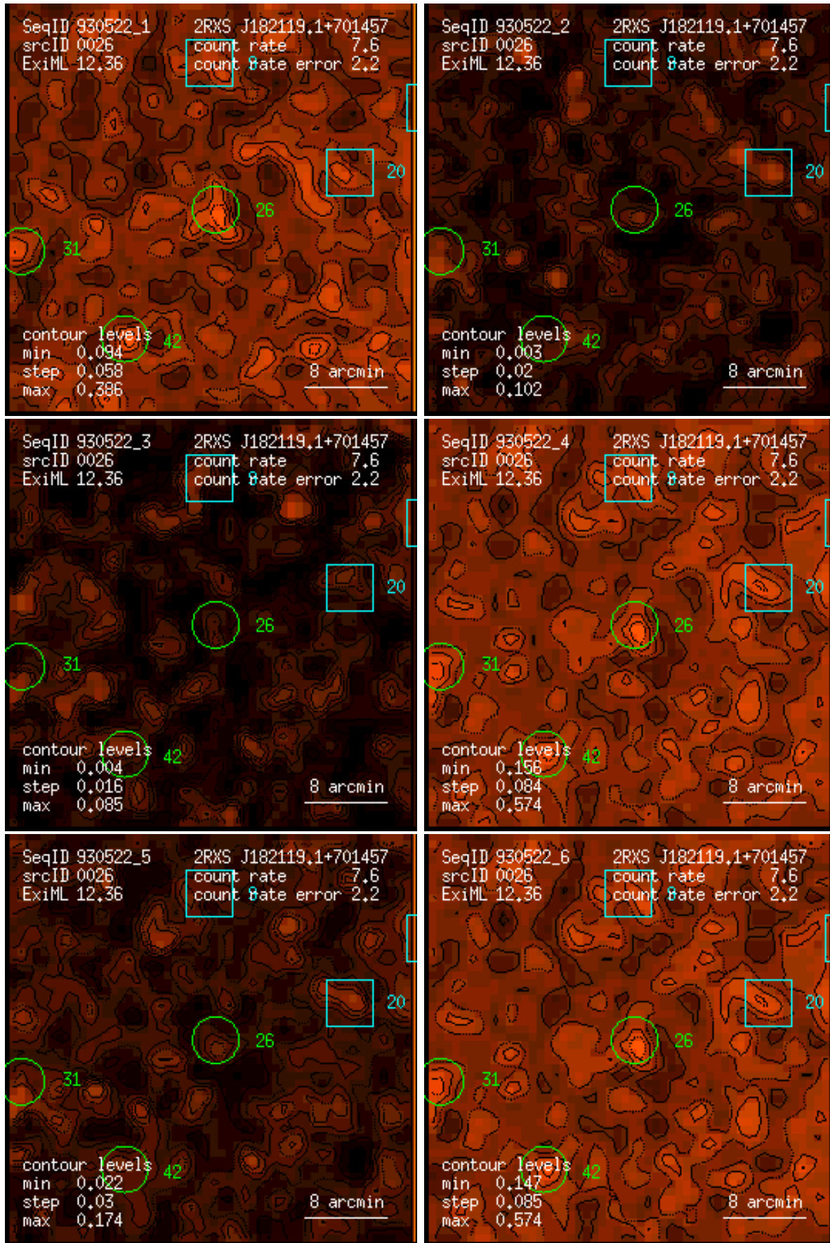
Figure 26: RASS 930522: detection 0026: band rate images, Gaussian filter: (1) PSPC channels 11 – 41, (2) 52 – 90, (3) 91 – 201, (4) 11 – 235, (5) 52 – 201, (6) 11 – 201. Broad band rates in counts/ks. Band rate contour levels in counts/ks/arcmin 2 .
