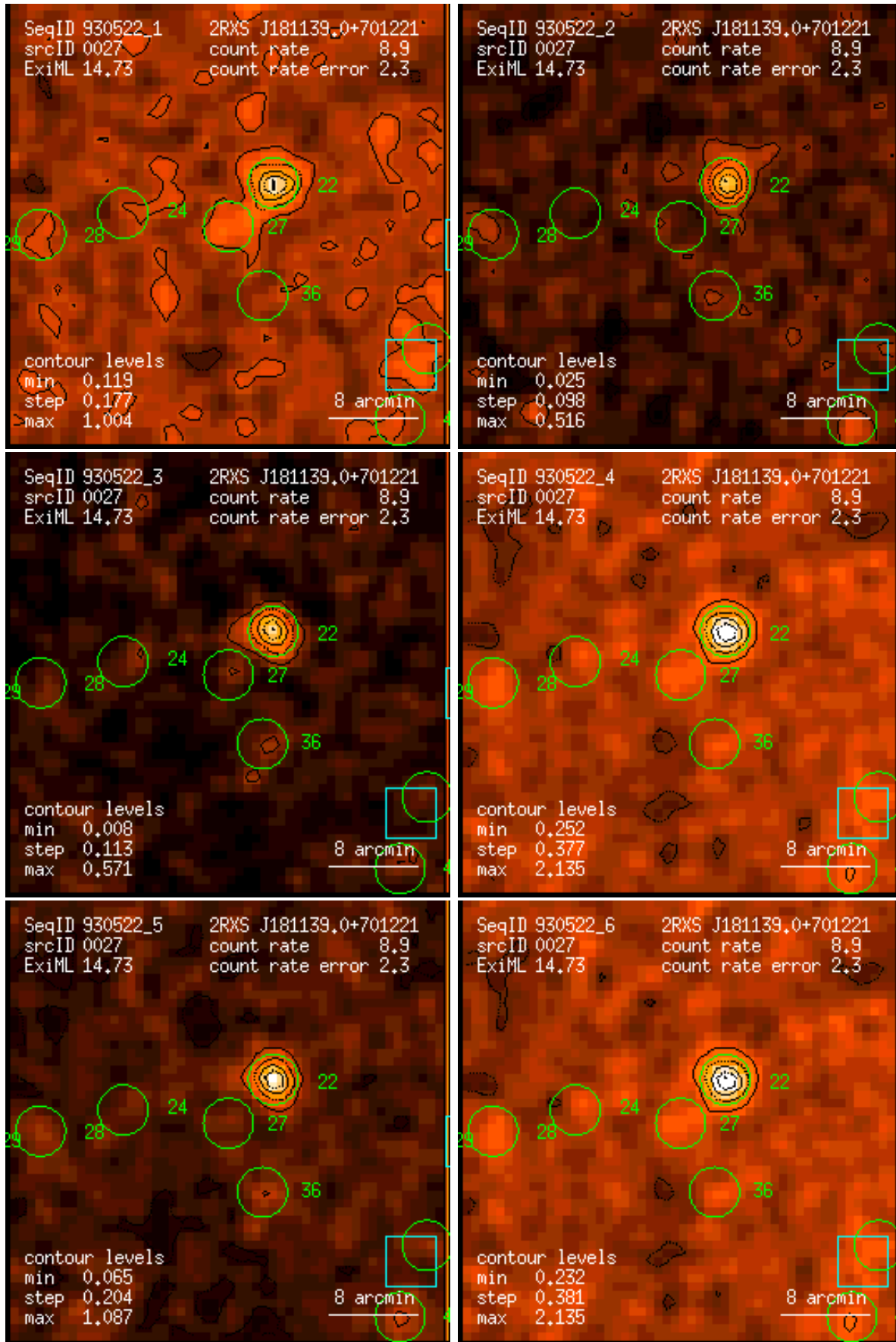
Figure 27: RASS 930522: detection 0027: band rate images, Gaussian filter: (1) PSPC channels 11 – 41, (2) 52 – 90, (3) 91 – 201, (4) 11 – 235, (5) 52 – 201, (6) 11 – 201. Broad band rates in counts/ks. Band rate contour levels in counts/ks/arcmin 2 .
