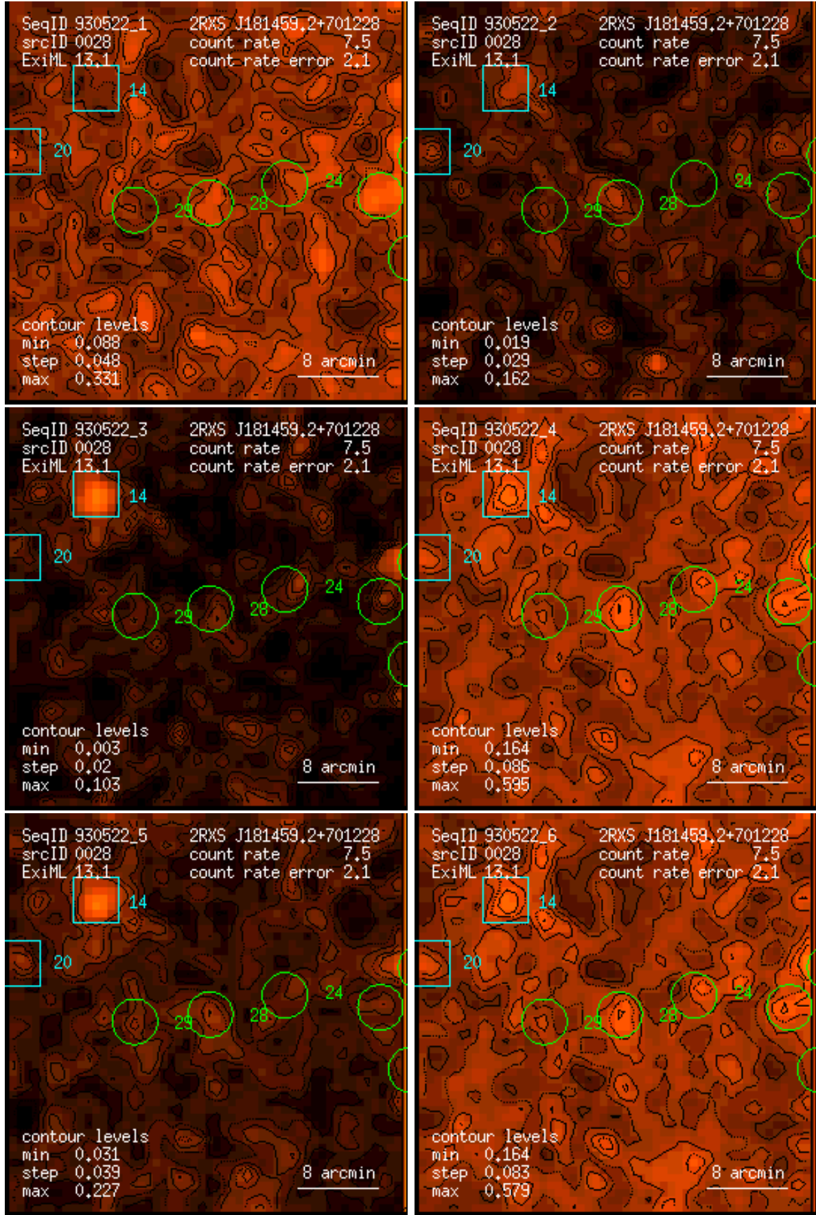
Figure 28: RASS 930522: detection 0028: band rate images, Gaussian filter: (1) PSPC channels 11 – 41, (2) 52 – 90, (3) 91 – 201, (4) 11 – 235, (5) 52 – 201, (6) 11 – 201. Broad band rates in counts/ks. Band rate contour levels in counts/ks/arcmin 2 .
