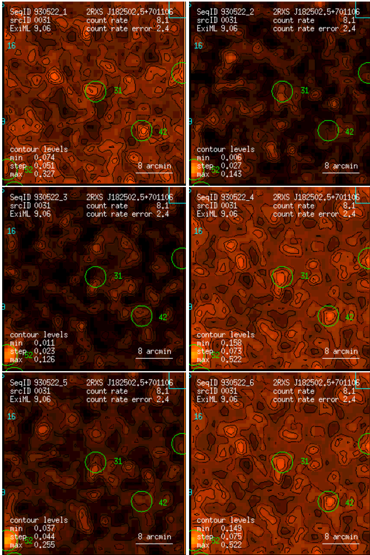
Figure 31: RASS 930522: detection 0031: band rate images, Gaussian filter: (1) PSPC channels 11 – 41, (2) 52 – 90, (3) 91 – 201, (4) 11 – 235, (5) 52 – 201, (6) 11 – 201. Broad band rates in counts/ks. Band rate contour levels in counts/ks/arcmin 2 .
