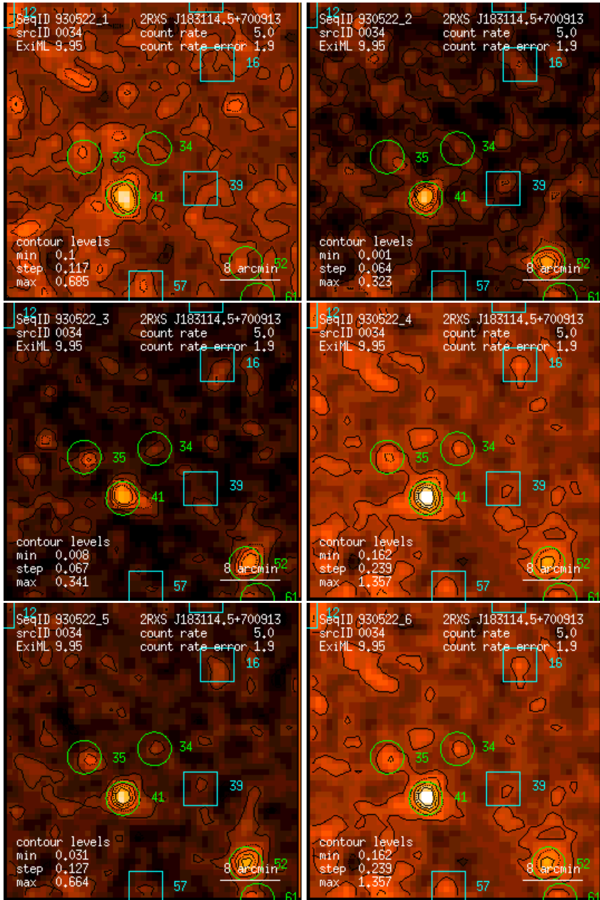
Figure 34: RASS 930522: detection 0034: band rate images, Gaussian filter: (1) PSPC channels 11 – 41, (2) 52 – 90, (3) 91 – 201, (4) 11 – 235, (5) 52 – 201, (6) 11 – 201. Broad band rates in counts/ks. Band rate contour levels in counts/ks/arcmin 2 .
