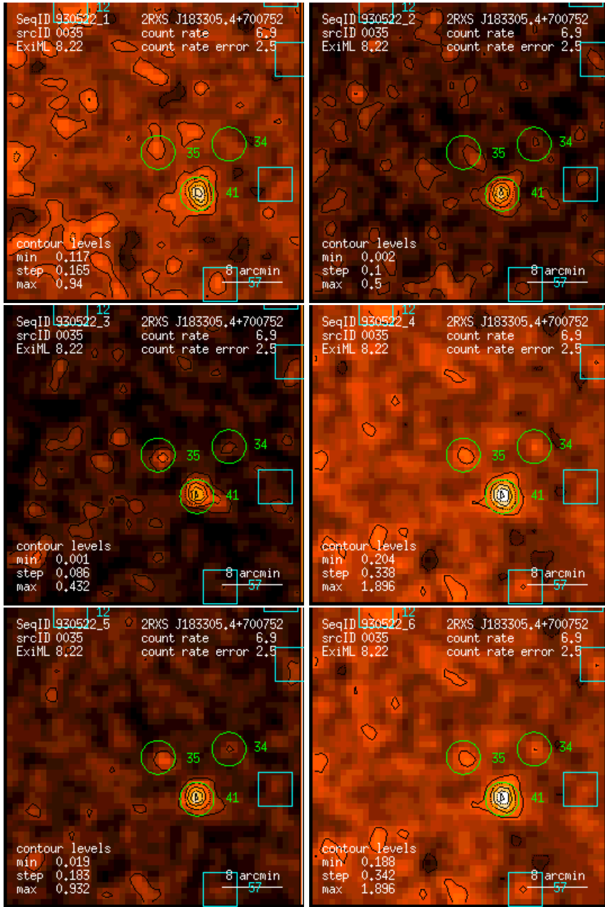
Figure 35: RASS 930522: detection 0035: band rate images, Gaussian filter: (1) PSPC channels 11 – 41, (2) 52 – 90, (3) 91 – 201, (4) 11 – 235, (5) 52 – 201, (6) 11 – 201. Broad band rates in counts/ks. Band rate contour levels in counts/ks/arcmin 2 .
