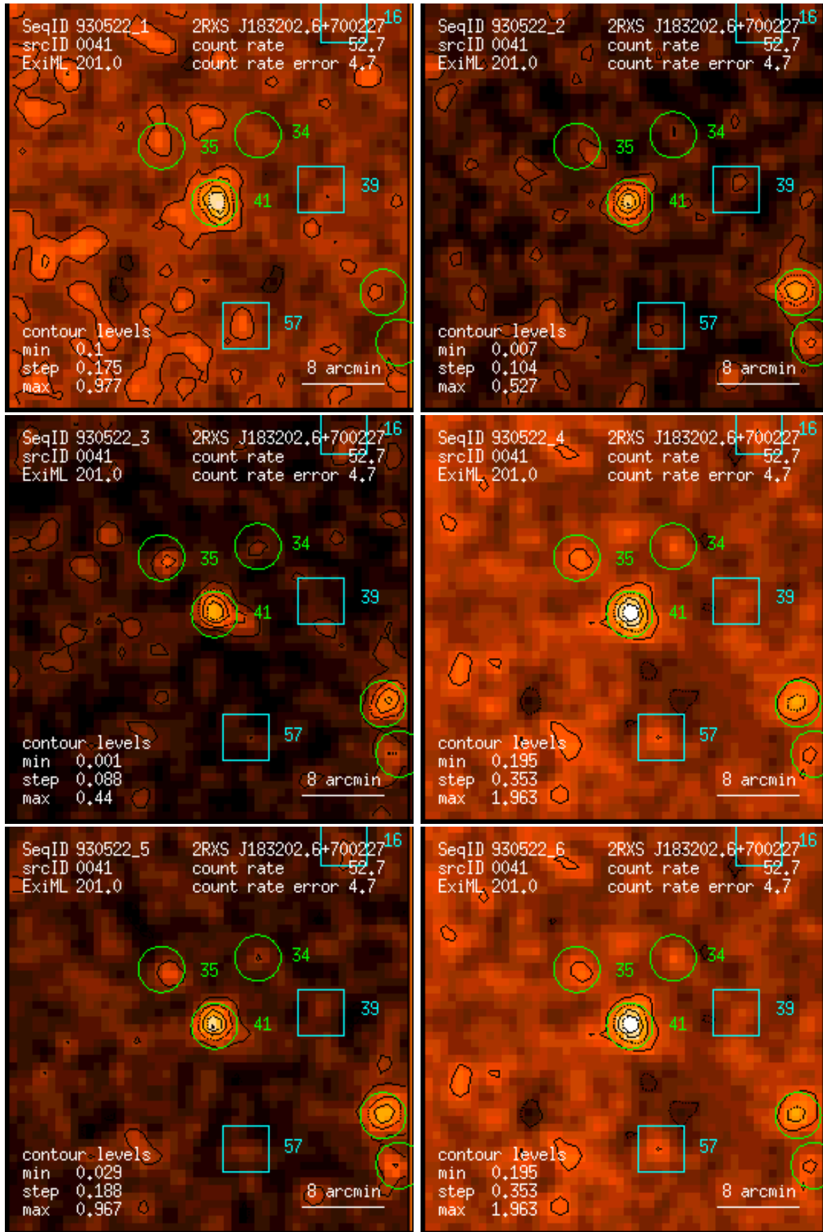
Figure 41: RASS 930522: detection 0041: band rate images, Gaussian filter: (1) PSPC channels 11 – 41, (2) 52 – 90, (3) 91 – 201, (4) 11 – 235, (5) 52 – 201, (6) 11 – 201. Broad band rates in counts/ks. Band rate contour levels in counts/ks/arcmin 2 .
