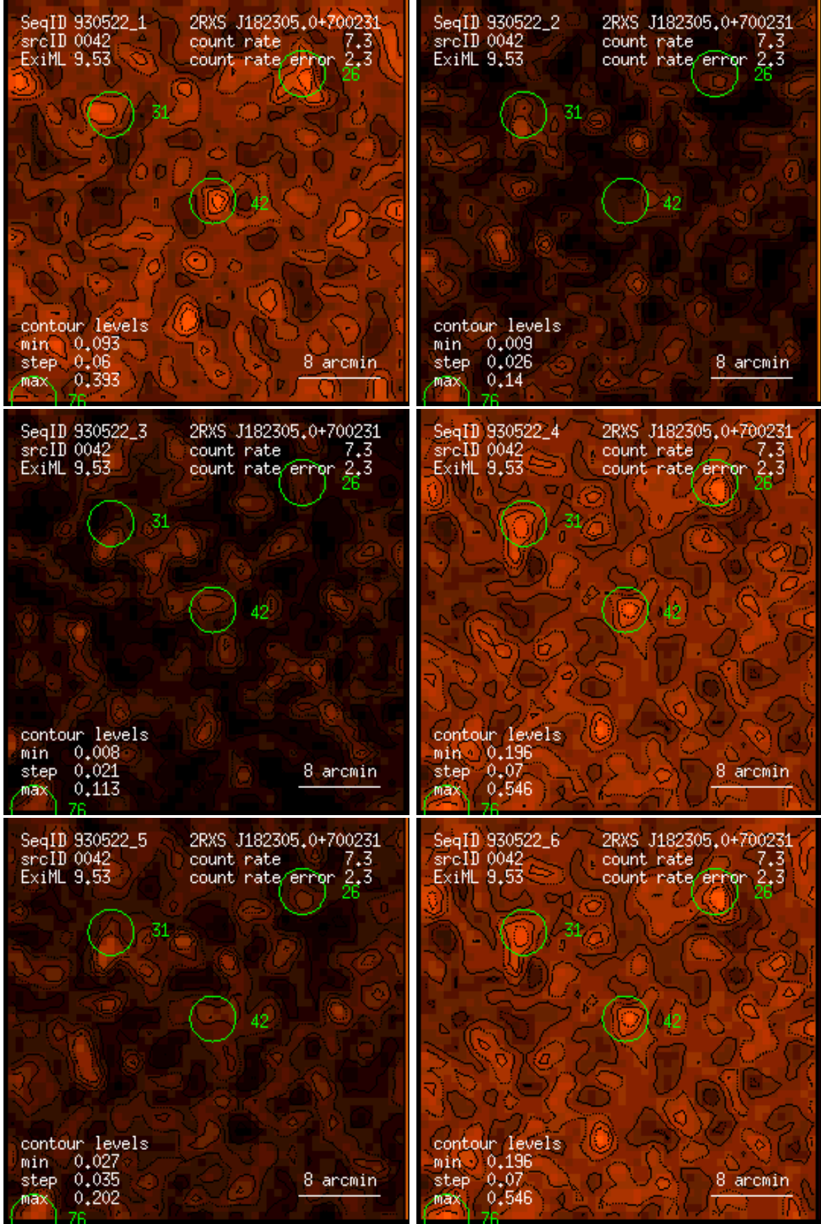
Figure 42: RASS 930522: detection 0042: band rate images, Gaussian filter: (1) PSPC channels 11 – 41, (2) 52 – 90, (3) 91 – 201, (4) 11 – 235, (5) 52 – 201, (6) 11 – 201. Broad band rates in counts/ks. Band rate contour levels in counts/ks/arcmin 2 .
