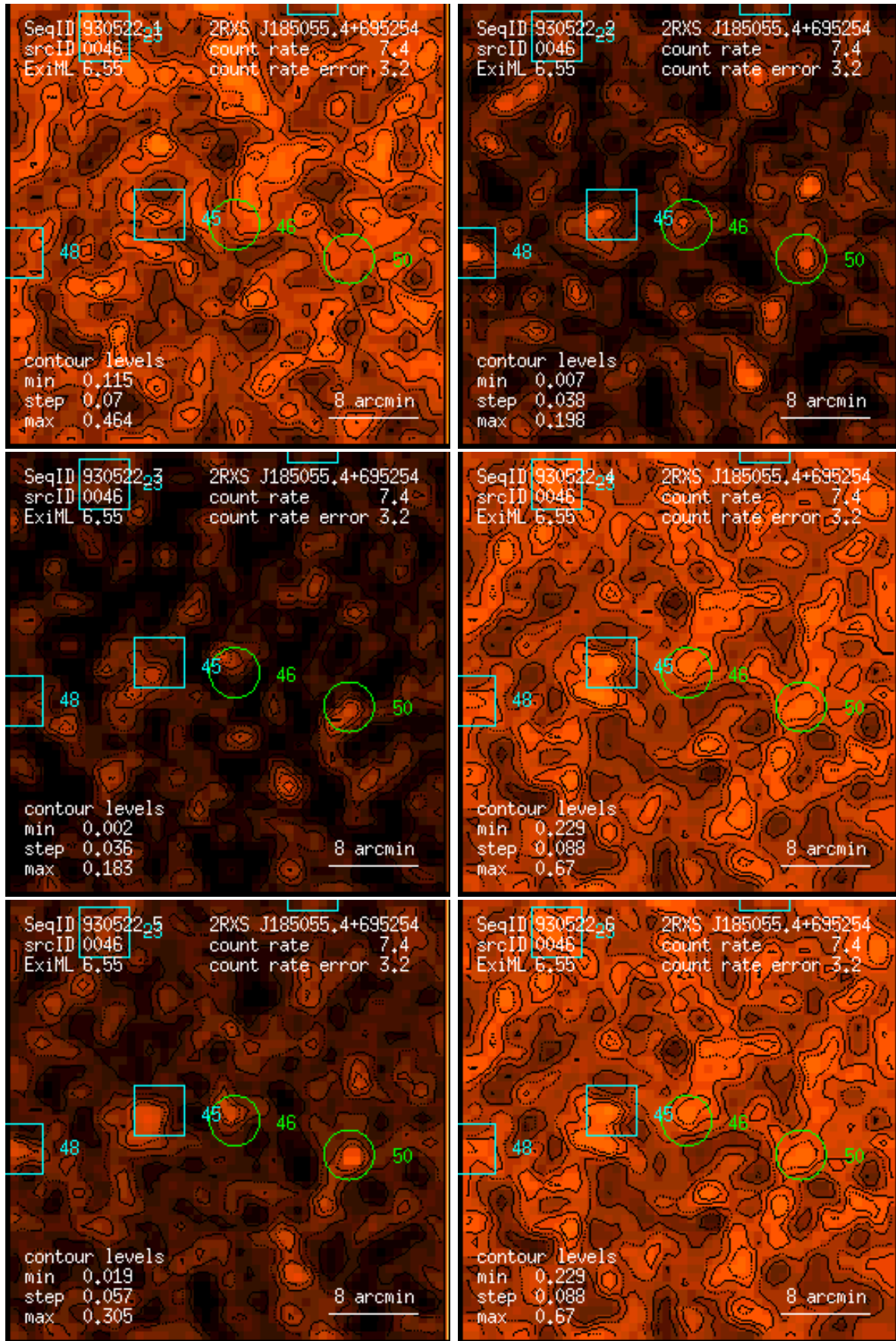
Figure 46: RASS 930522: detection 0046: band rate images, Gaussian filter: (1) PSPC channels 11 – 41, (2) 52 – 90, (3) 91 – 201, (4) 11 – 235, (5) 52 – 201, (6) 11 – 201. Broad band rates in counts/ks. Band rate contour levels in counts/ks/arcmin 2 .
