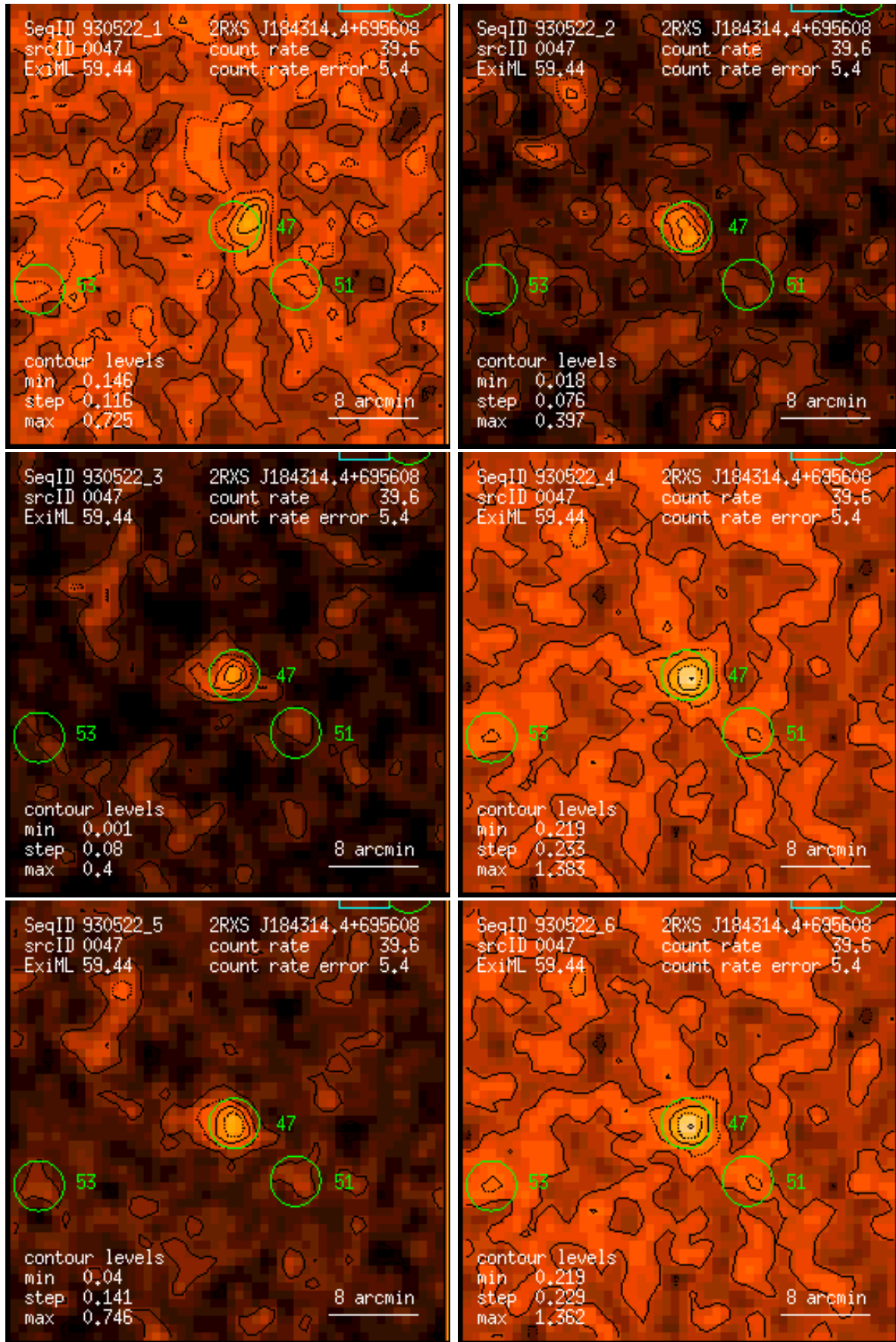
Figure 47: RASS 930522: detection 0047: band rate images, Gaussian filter: (1) PSPC channels 11 – 41, (2) 52 – 90, (3) 91 – 201, (4) 11 – 235, (5) 52 – 201, (6) 11 – 201. Broad band rates in counts/ks. Band rate contour levels in counts/ks/arcmin 2 .
