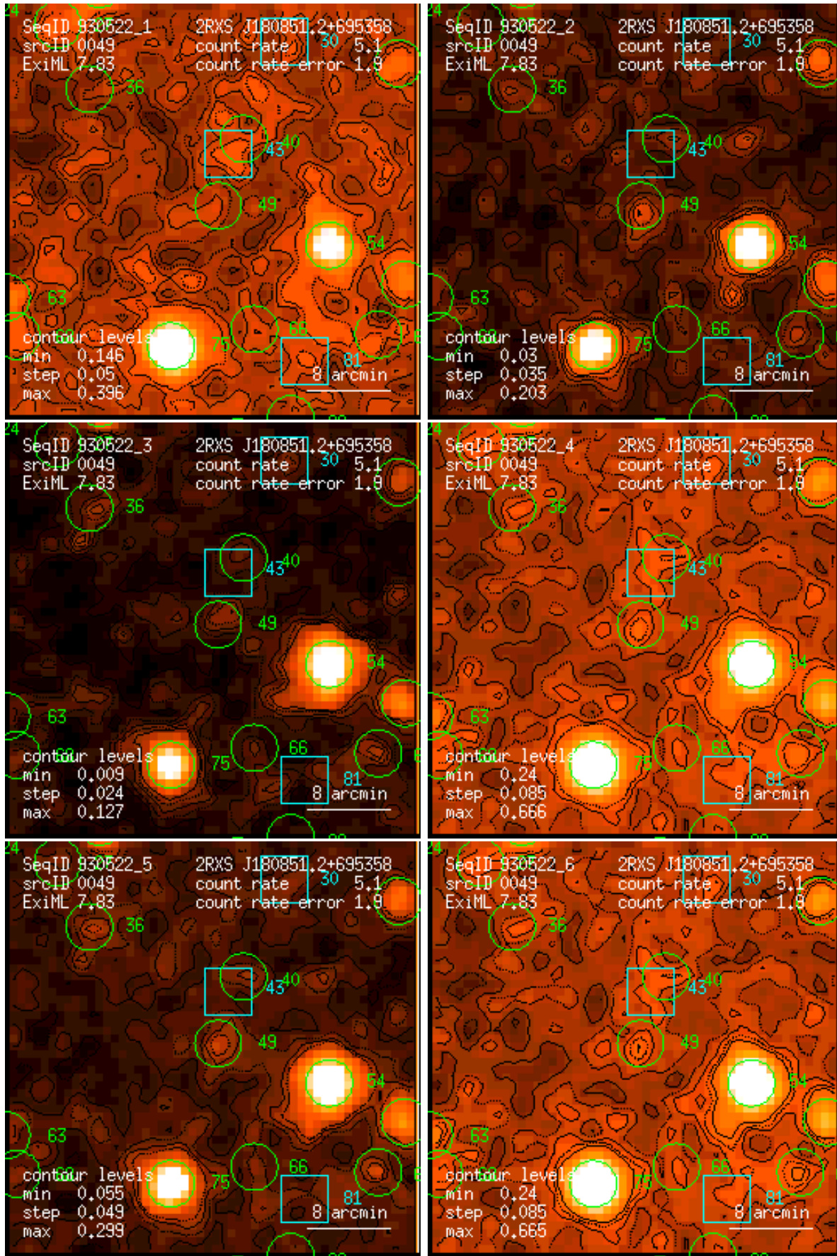
Figure 49: RASS 930522: detection 0049: band rate images, Gaussian filter: (1) PSPC channels 11 – 41, (2) 52 – 90, (3) 91 – 201, (4) 11 – 235, (5) 52 – 201, (6) 11 – 201. Broad band rates in counts/ks. Band rate contour levels in counts/ks/arcmin 2 .
