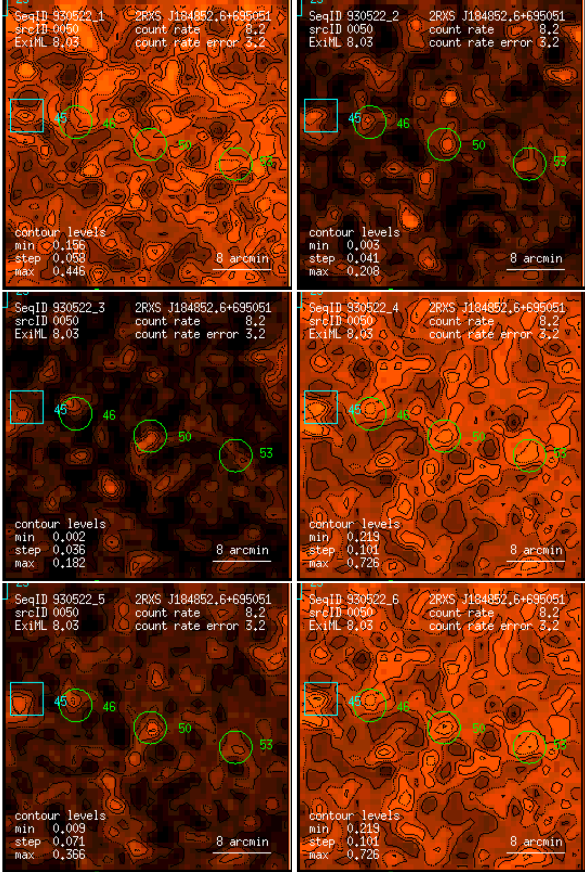
Figure 50: RASS 930522: detection 0050: band rate images, Gaussian filter: (1) PSPC channels 11 – 41, (2) 52 – 90, (3) 91 – 201, (4) 11 – 235, (5) 52 – 201, (6) 11 – 201. Broad band rates in counts/ks. Band rate contour levels in counts/ks/arcmin 2 .
