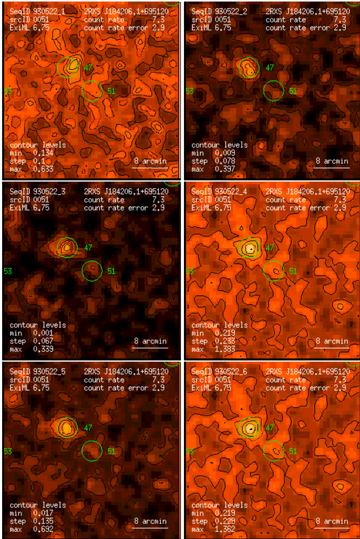
Figure 51: RASS 930522: detection 0051: band rate images, Gaussian filter: (1) PSPC channels 11 – 41, (2) 52 – 90, (3) 91 – 201, (4) 11 – 235, (5) 52 – 201, (6) 11 – 201. Broad band rates in counts/ks. Band rate contour levels in counts/ks/arcmin 2 .
