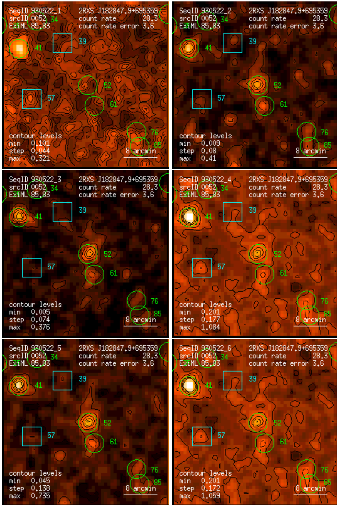
Figure 52: RASS 930522: detection 0052: band rate images, Gaussian filter: (1) PSPC channels 11 – 41, (2) 52 – 90, (3) 91 – 201, (4) 11 – 235, (5) 52 – 201, (6) 11 – 201. Broad band rates in counts/ks. Band rate contour levels in counts/ks/arcmin 2 .
