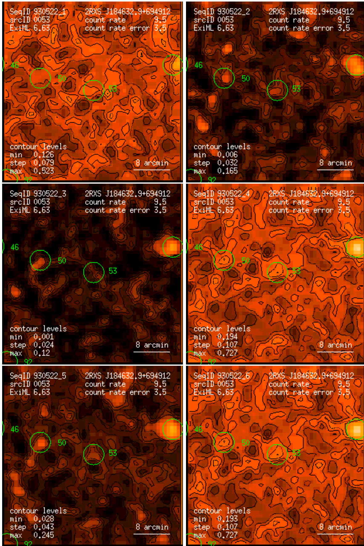
Figure 53: RASS 930522: detection 0053: band rate images, Gaussian filter: (1) PSPC channels 11 – 41, (2) 52 – 90, (3) 91 – 201, (4) 11 – 235, (5) 52 – 201, (6) 11 – 201. Broad band rates in counts/ks. Band rate contour levels in counts/ks/arcmin 2 .
