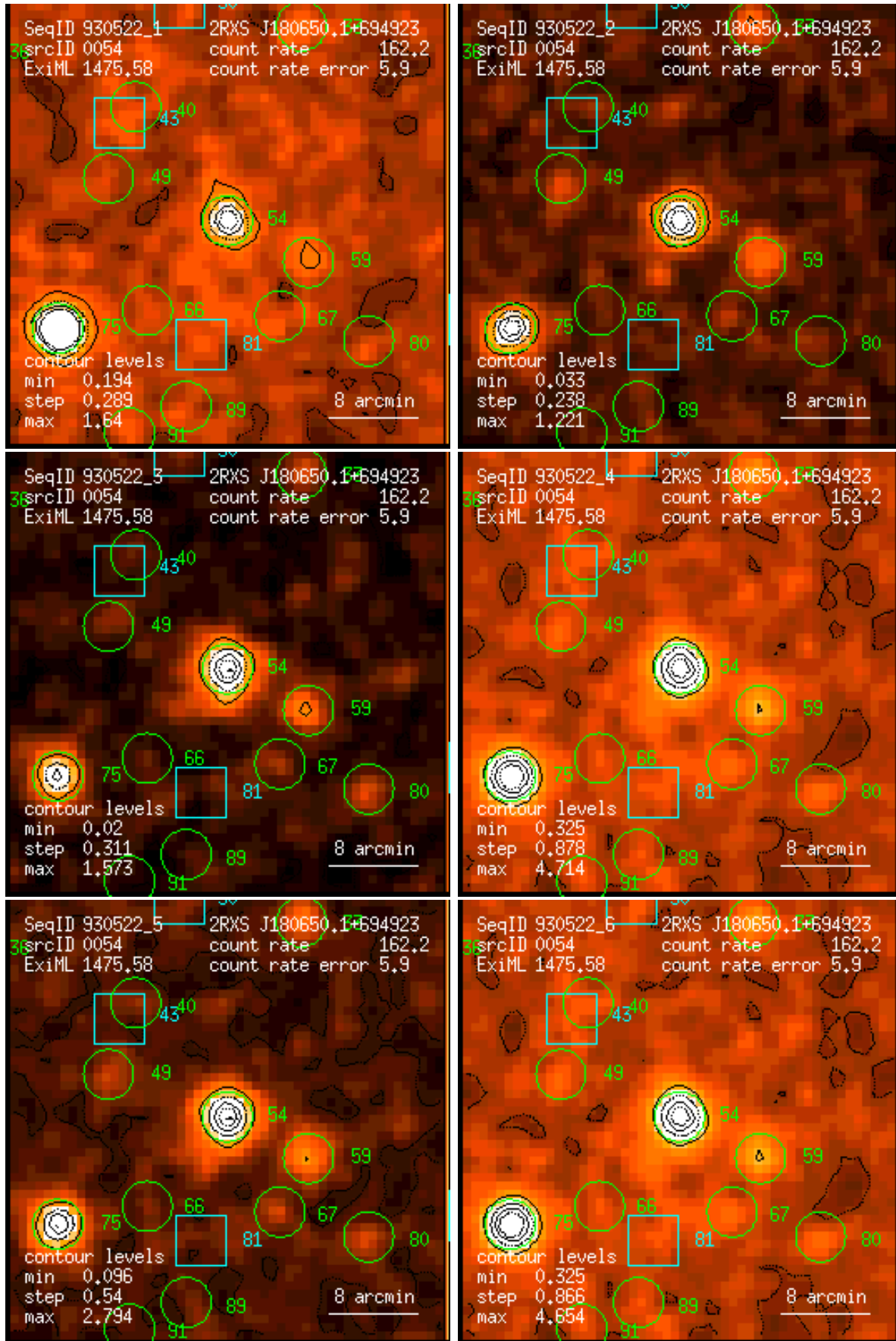
Figure 54: RASS 930522: detection 0054: band rate images, Gaussian filter: (1) PSPC channels 11 – 41, (2) 52 – 90, (3) 91 – 201, (4) 11 – 235, (5) 52 – 201, (6) 11 – 201. Broad band rates in counts/ks. Band rate contour levels in counts/ks/arcmin 2 .
