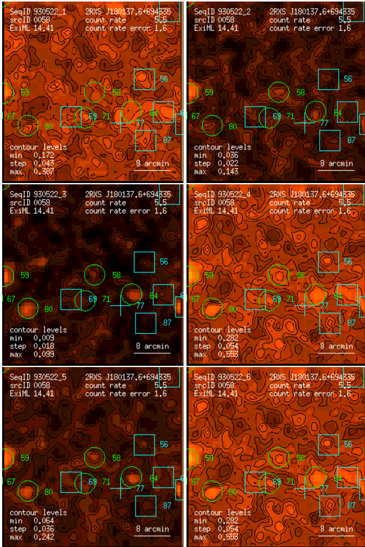
Figure 58: RASS 930522: detection 0058: band rate images, Gaussian filter: (1) PSPC channels 11 – 41, (2) 52 – 90, (3) 91 – 201, (4) 11 – 235, (5) 52 – 201, (6) 11 – 201. Broad band rates in counts/ks. Band rate contour levels in counts/ks/arcmin 2 .
