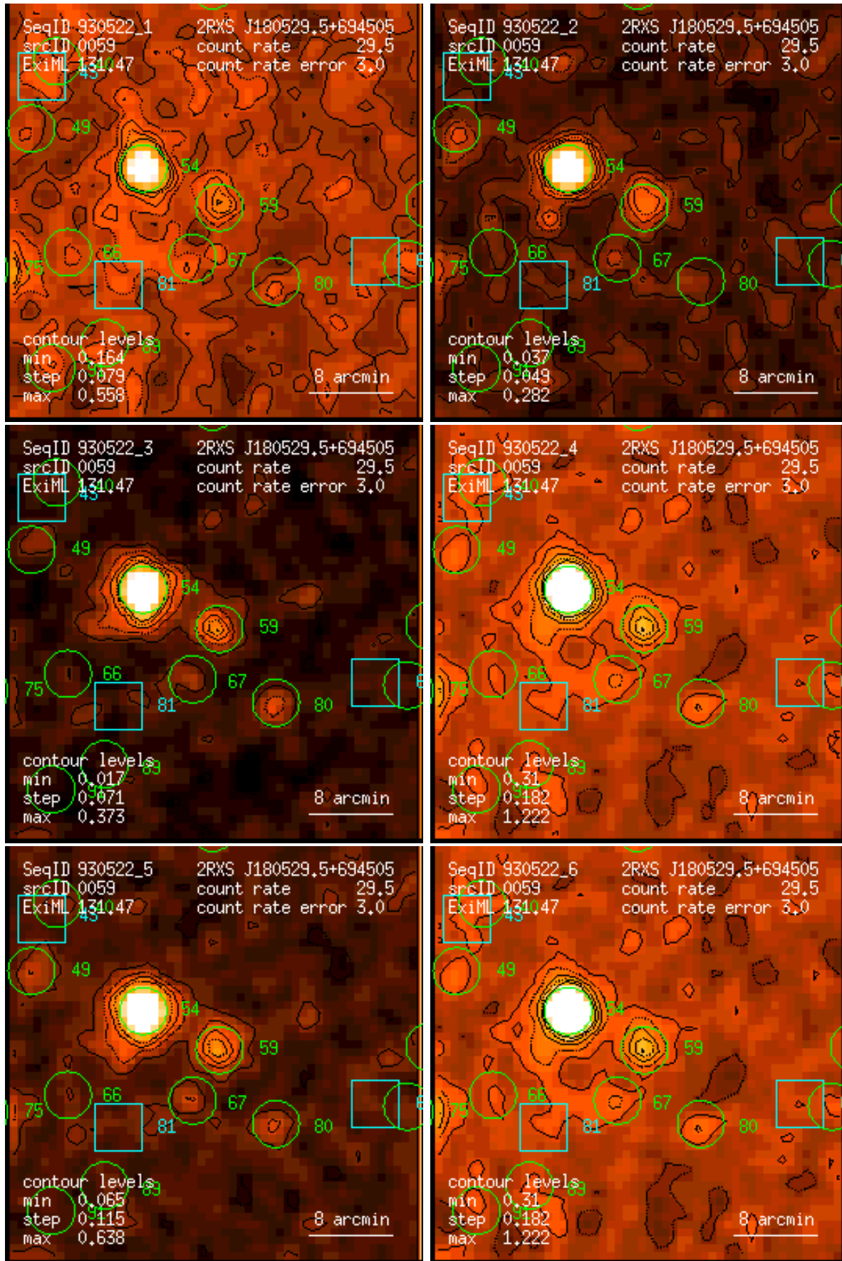
Figure 59: RASS 930522: detection 0059: band rate images, Gaussian filter: (1) PSPC channels 11 – 41, (2) 52 – 90, (3) 91 – 201, (4) 11 – 235, (5) 52 – 201, (6) 11 – 201. Broad band rates in counts/ks. Band rate contour levels in counts/ks/arcmin 2 .
