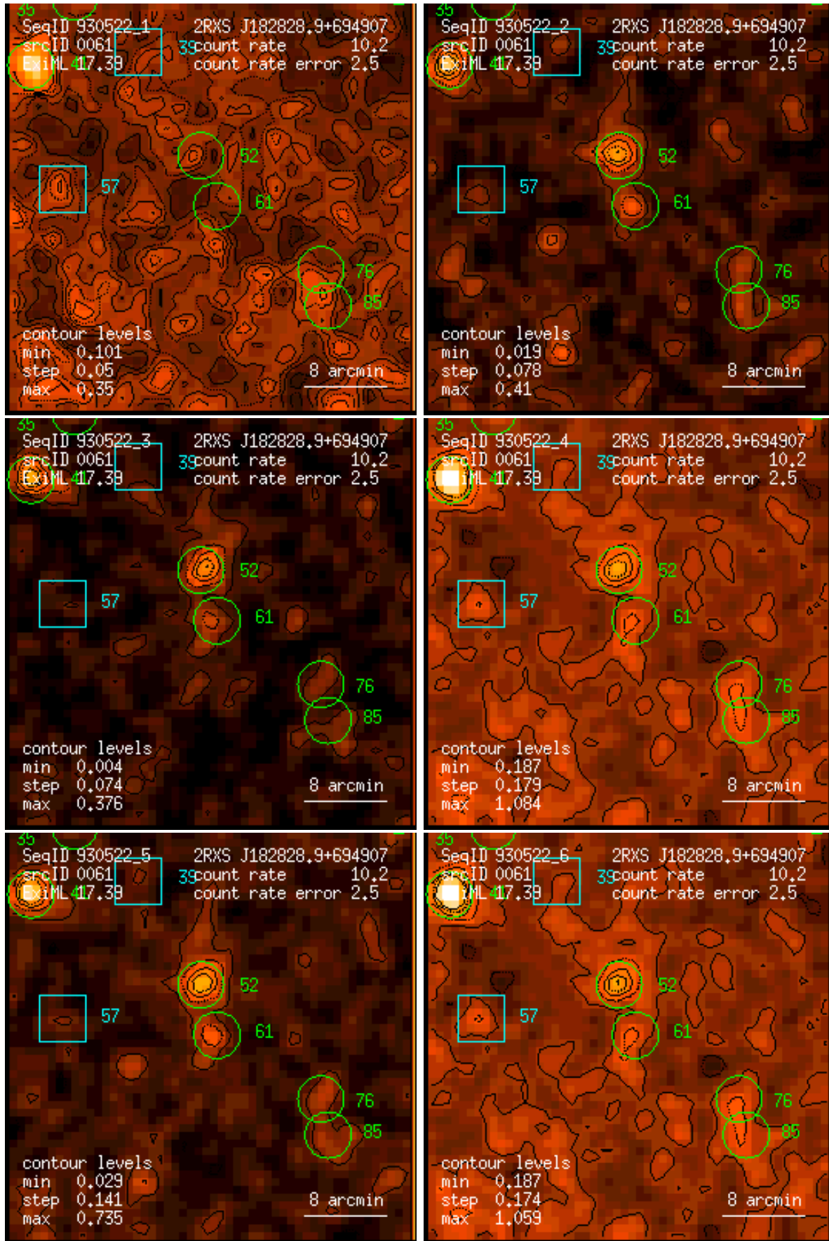
Figure 61: RASS 930522: detection 0061: band rate images, Gaussian filter: (1) PSPC channels 11 – 41, (2) 52 – 90, (3) 91 – 201, (4) 11 – 235, (5) 52 – 201, (6) 11 – 201. Broad band rates in counts/ks. Band rate contour levels in counts/ks/arcmin 2 .
