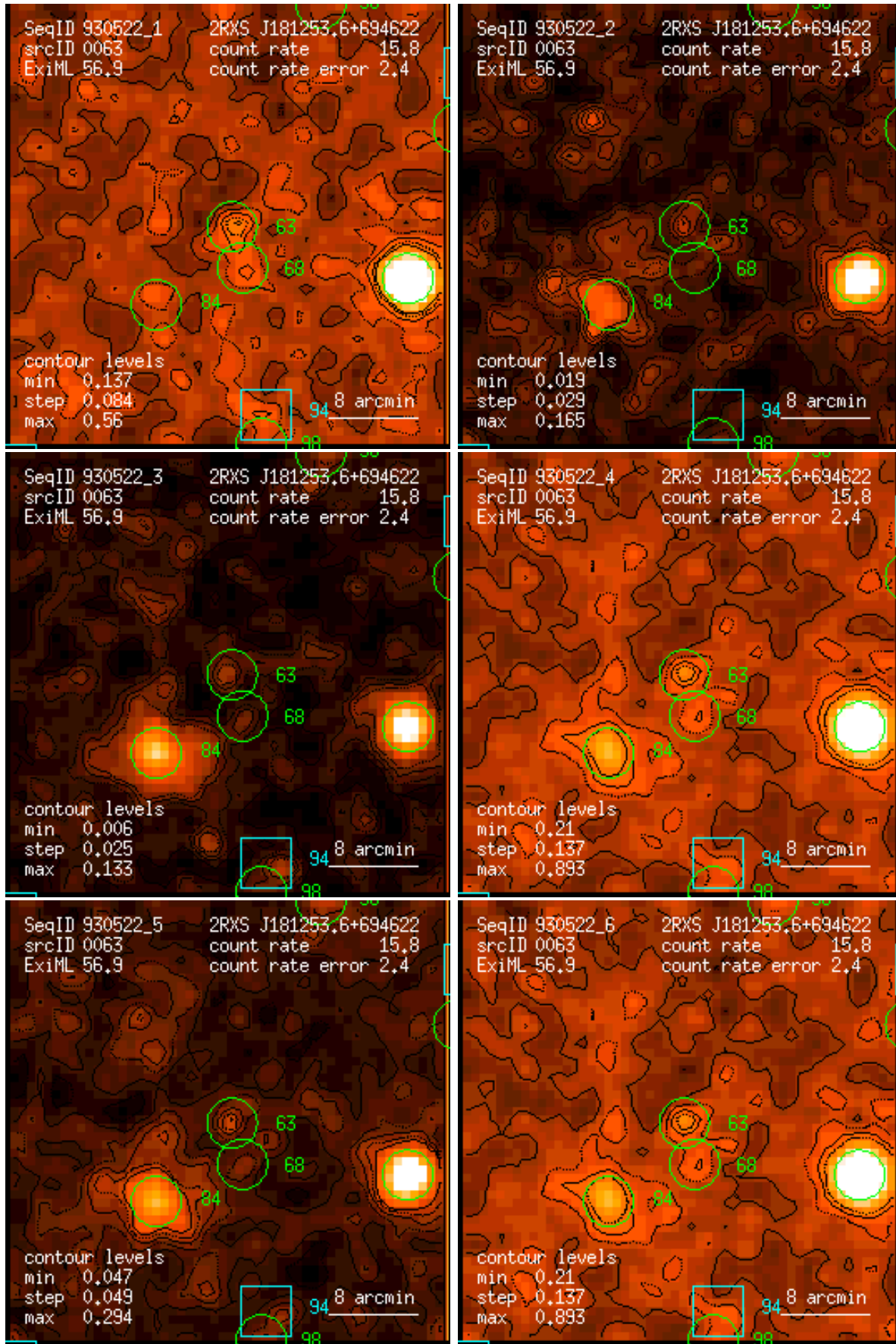
Figure 63: RASS 930522: detection 0063: band rate images, Gaussian filter: (1) PSPC channels 11 – 41, (2) 52 – 90, (3) 91 – 201, (4) 11 – 235, (5) 52 – 201, (6) 11 – 201. Broad band rates in counts/ks. Band rate contour levels in counts/ks/arcmin 2 .
