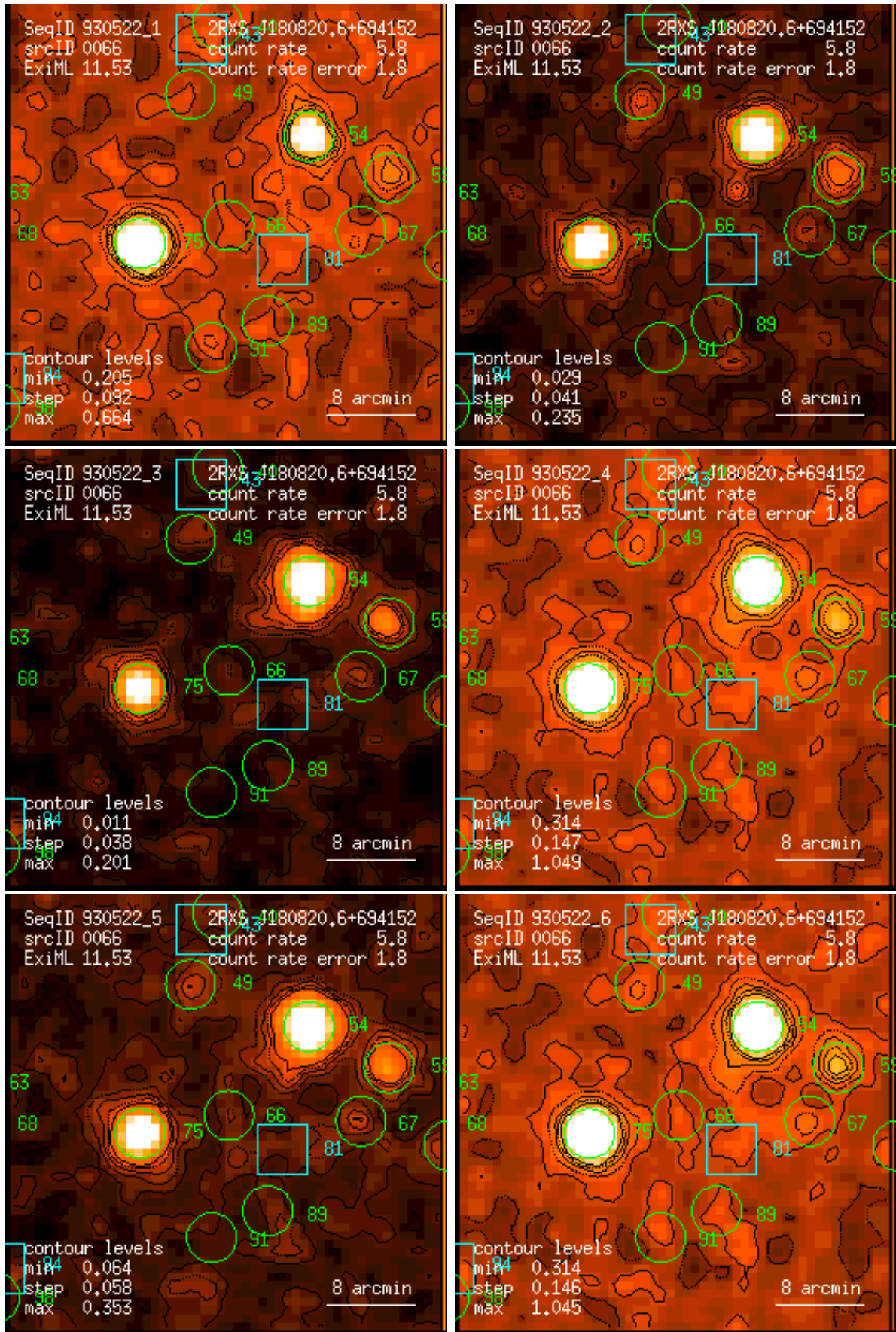
Figure 66: RASS 930522: detection 0066: band rate images, Gaussian filter: (1) PSPC channels 11 – 41, (2) 52 – 90, (3) 91 – 201, (4) 11 – 235, (5) 52 – 201, (6) 11 – 201. Broad band rates in counts/ks. Band rate contour levels in counts/ks/arcmin 2 .
