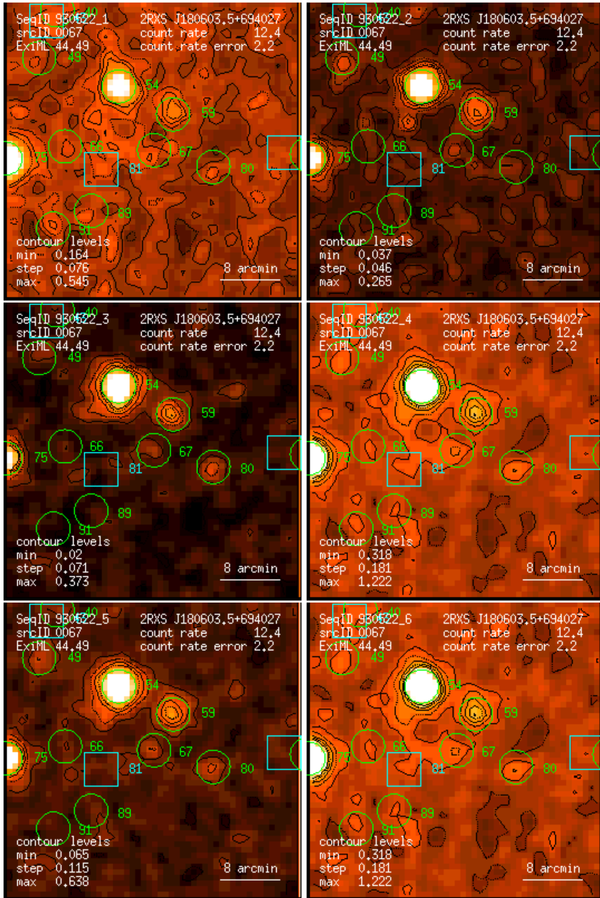
Figure 67: RASS 930522: detection 0067: band rate images, Gaussian filter: (1) PSPC channels 11 – 41, (2) 52 – 90, (3) 91 – 201, (4) 11 – 235, (5) 52 – 201, (6) 11 – 201. Broad band rates in counts/ks. Band rate contour levels in counts/ks/arcmin 2 .
