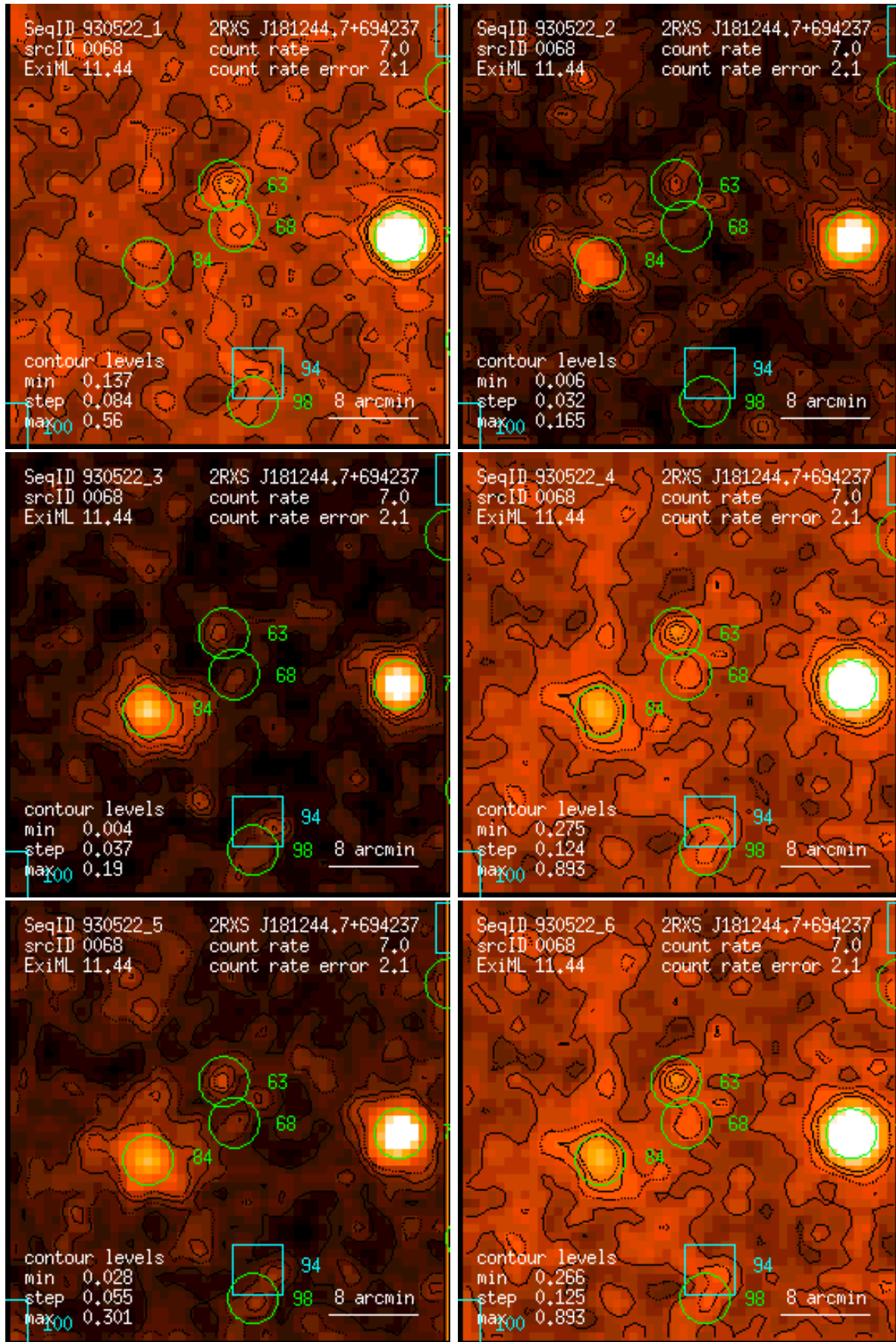
Figure 68: RASS 930522: detection 0068: band rate images, Gaussian filter: (1) PSPC channels 11 – 41, (2) 52 – 90, (3) 91 – 201, (4) 11 – 235, (5) 52 – 201, (6) 11 – 201. Broad band rates in counts/ks. Band rate contour levels in counts/ks/arcmin 2 .
