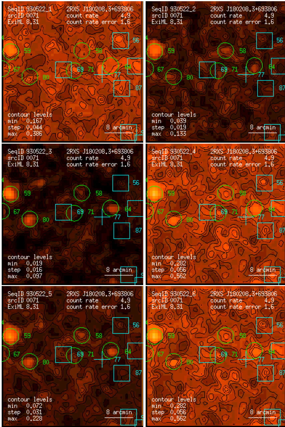
Figure 71: RASS 930522: detection 0071: band rate images, Gaussian filter: (1) PSPC channels 11 – 41, (2) 52 – 90, (3) 91 – 201, (4) 11 – 235, (5) 52 – 201, (6) 11 – 201. Broad band rates in counts/ks. Band rate contour levels in counts/ks/arcmin 2 .
