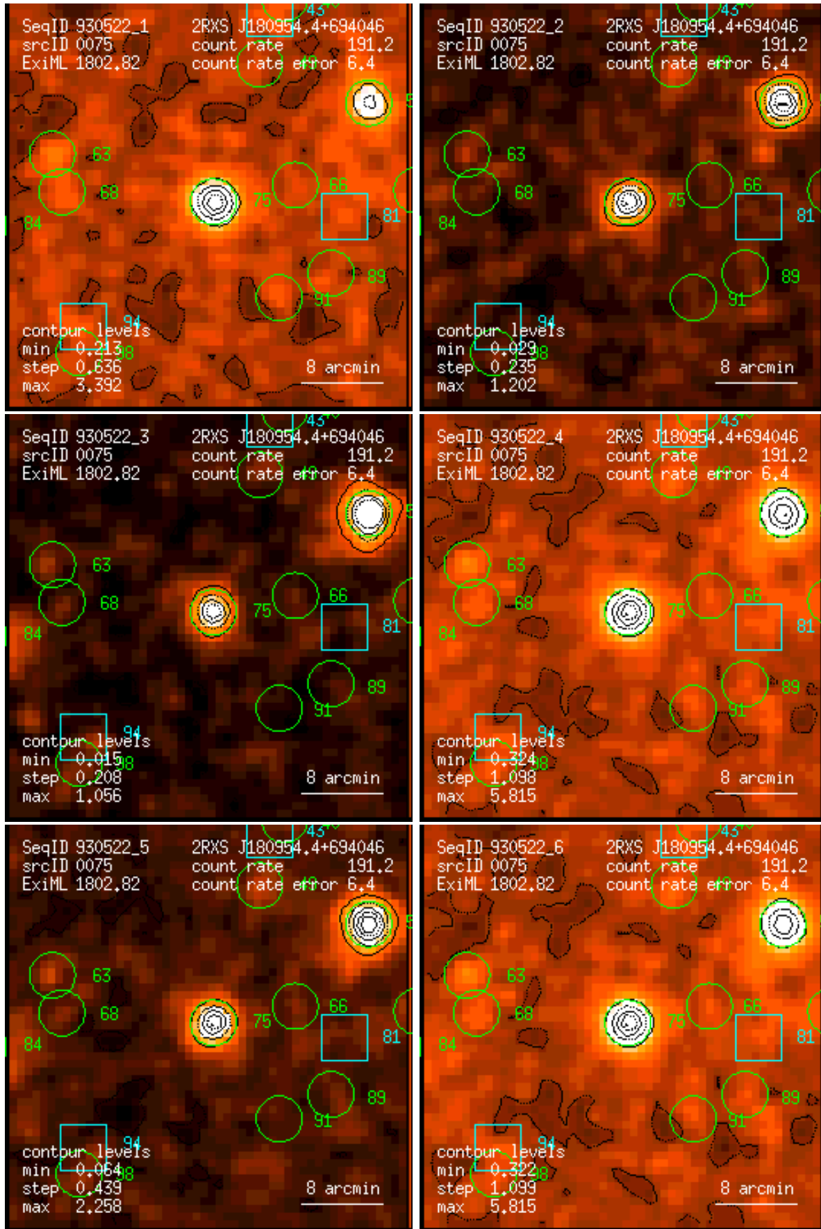
Figure 75: RASS 930522: detection 0075: band rate images, Gaussian filter: (1) PSPC channels 11 – 41, (2) 52 – 90, (3) 91 – 201, (4) 11 – 235, (5) 52 – 201, (6) 11 – 201. Broad band rates in counts/ks. Band rate contour levels in counts/ks/arcmin 2 .
