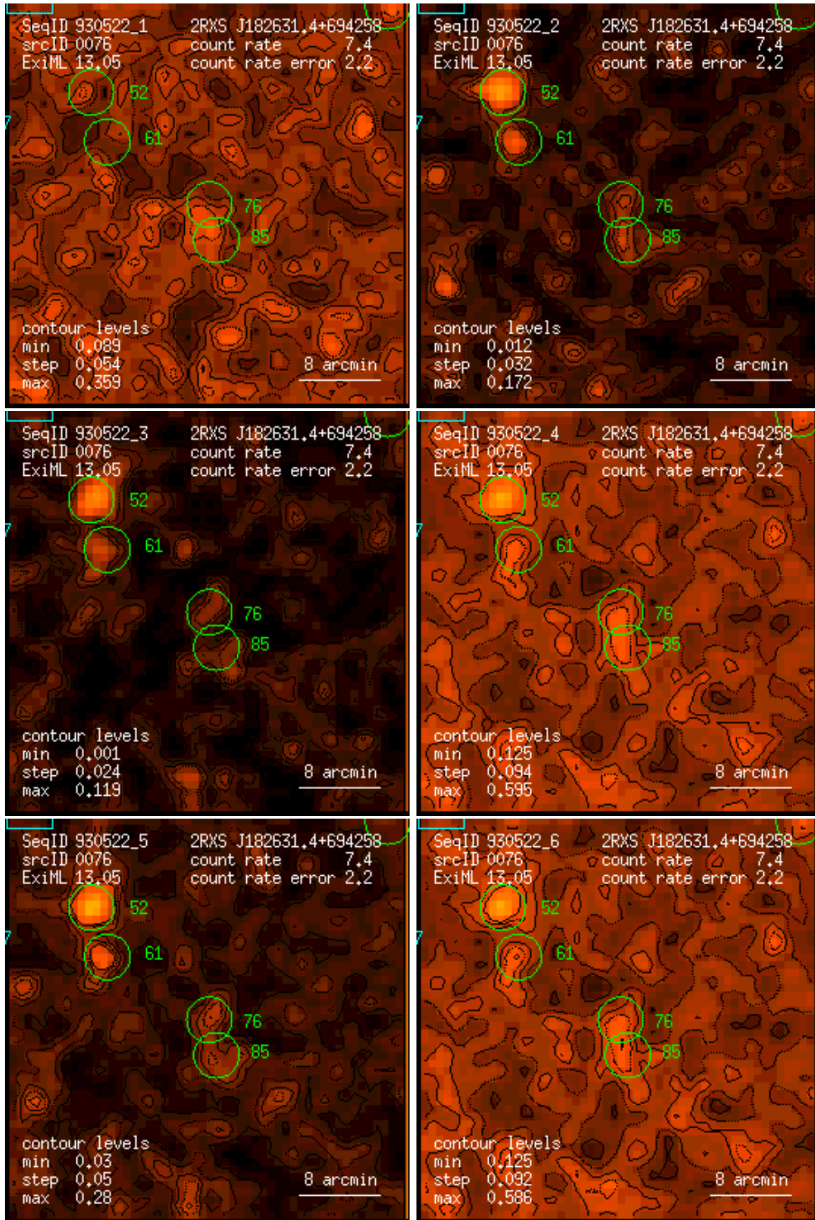
Figure 76: RASS 930522: detection 0076: band rate images, Gaussian filter: (1) PSPC channels 11 – 41, (2) 52 – 90, (3) 91 – 201, (4) 11 – 235, (5) 52 – 201, (6) 11 – 201. Broad band rates in counts/ks. Band rate contour levels in counts/ks/arcmin 2 .
