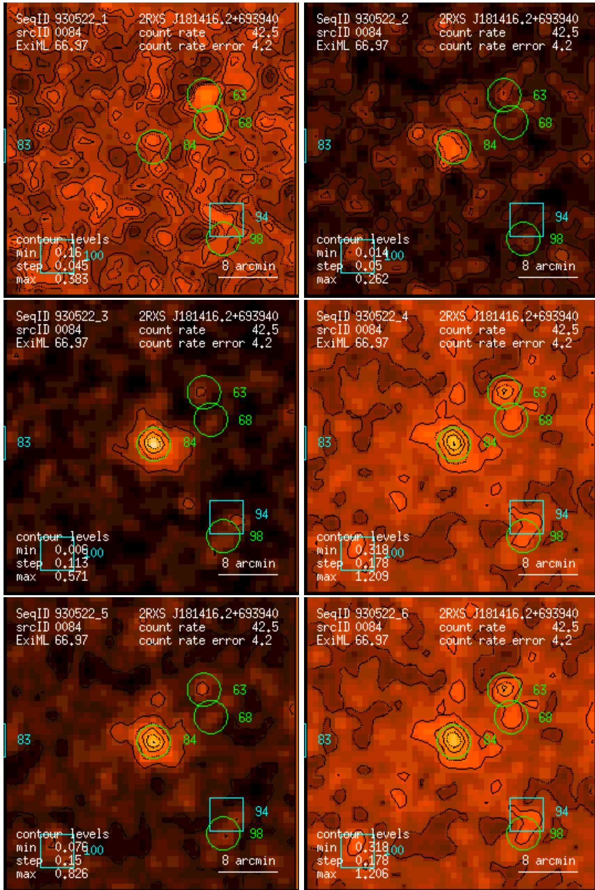
Figure 84: RASS 930522: detection 0084: band rate images, Gaussian filter: (1) PSPC channels 11 – 41, (2) 52 – 90, (3) 91 – 201, (4) 11 – 235, (5) 52 – 201, (6) 11 – 201. Broad band rates in counts/ks. Band rate contour levels in counts/ks/arcmin 2 .
