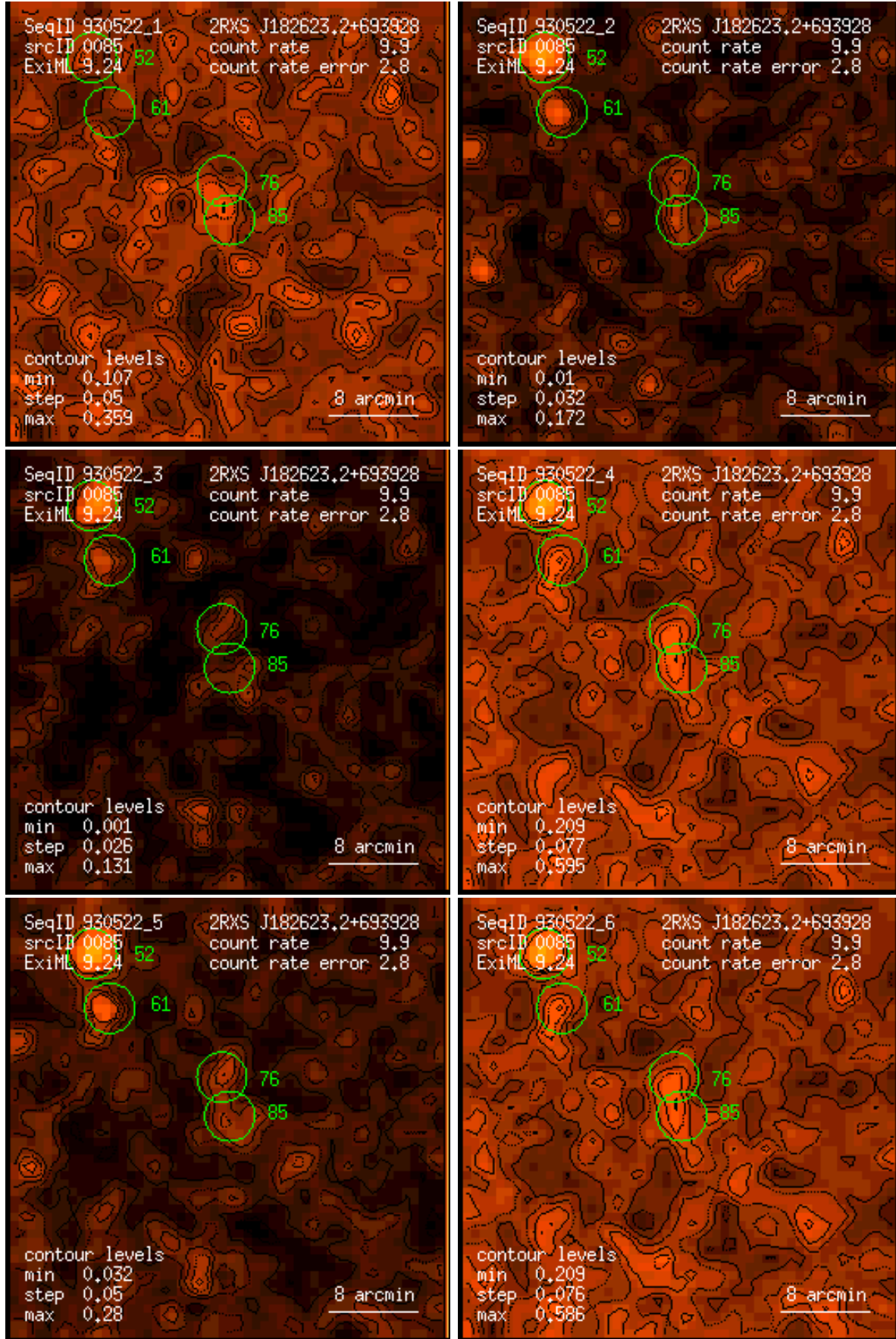
Figure 85: RASS 930522: detection 0085: band rate images, Gaussian filter: (1) PSPC channels 11 – 41, (2) 52 – 90, (3) 91 – 201, (4) 11 – 235, (5) 52 – 201, (6) 11 – 201. Broad band rates in counts/ks. Band rate contour levels in counts/ks/arcmin 2 .
