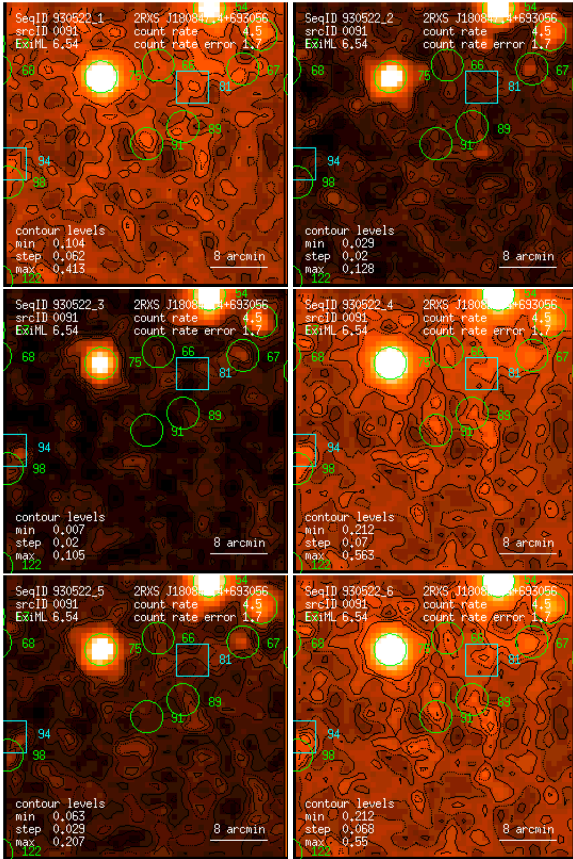
Figure 91: RASS 930522: detection 0091: band rate images, Gaussian filter: (1) PSPC channels 11 – 41, (2) 52 – 90, (3) 91 – 201, (4) 11 – 235, (5) 52 – 201, (6) 11 – 201. Broad band rates in counts/ks. Band rate contour levels in counts/ks/arcmin 2 .
