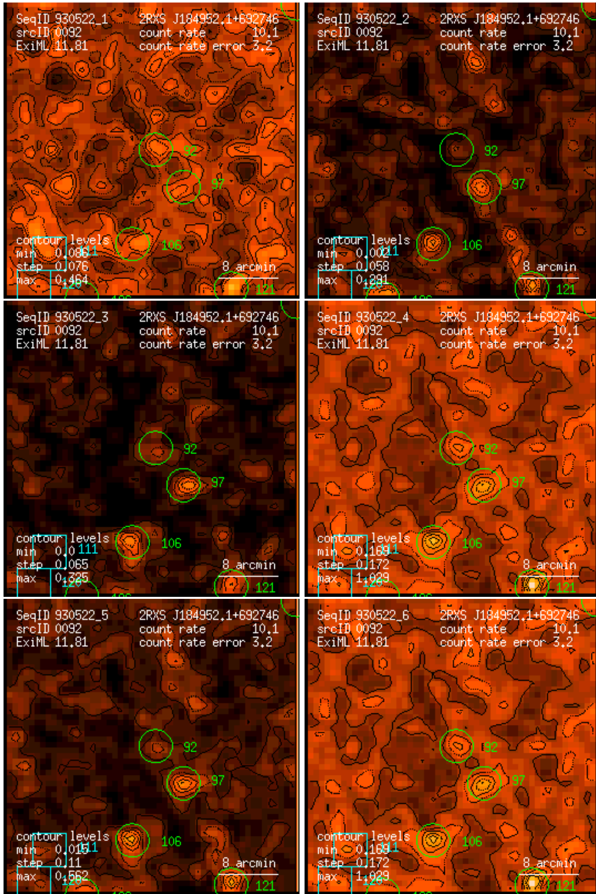
Figure 92: RASS 930522: detection 0092: band rate images, Gaussian filter: (1) PSPC channels 11 – 41, (2) 52 – 90, (3) 91 – 201, (4) 11 – 235, (5) 52 – 201, (6) 11 – 201. Broad band rates in counts/ks. Band rate contour levels in counts/ks/arcmin 2 .
