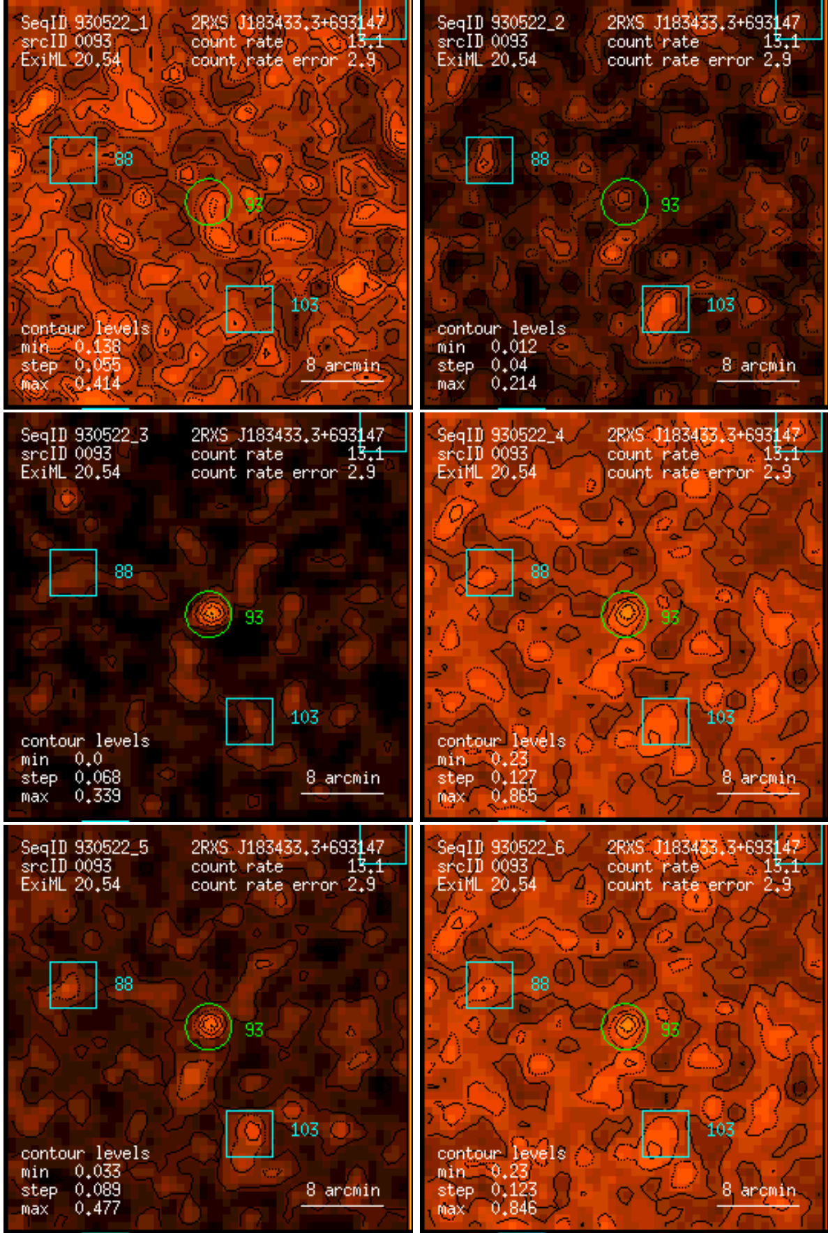
Figure 93: RASS 930522: detection 0093: band rate images, Gaussian filter: (1) PSPC channels 11 – 41, (2) 52 – 90, (3) 91 – 201, (4) 11 – 235, (5) 52 – 201, (6) 11 – 201. Broad band rates in counts/ks. Band rate contour levels in counts/ks/arcmin 2 .
