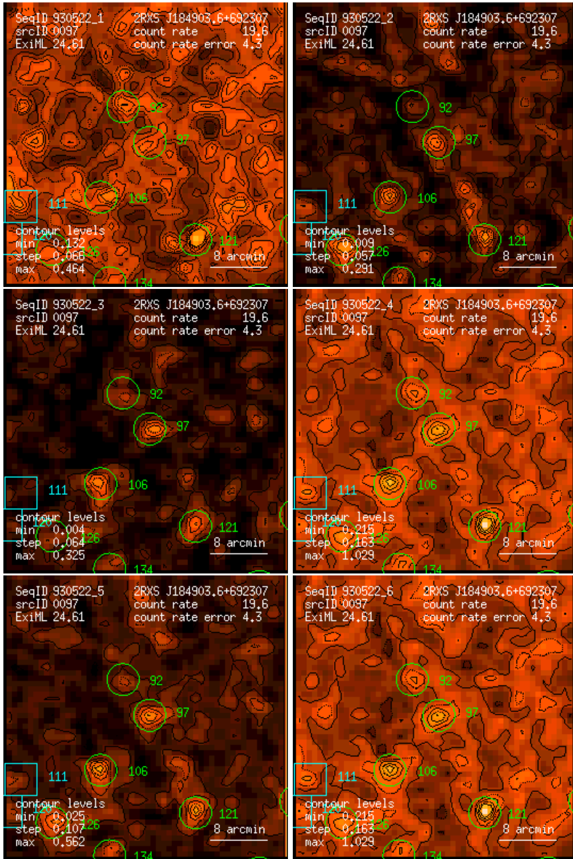
Figure 97: RASS 930522: detection 0097: band rate images, Gaussian filter: (1) PSPC channels 11 – 41, (2) 52 – 90, (3) 91 – 201, (4) 11 – 235, (5) 52 – 201, (6) 11 – 201. Broad band rates in counts/ks. Band rate contour levels in counts/ks/arcmin 2 .
