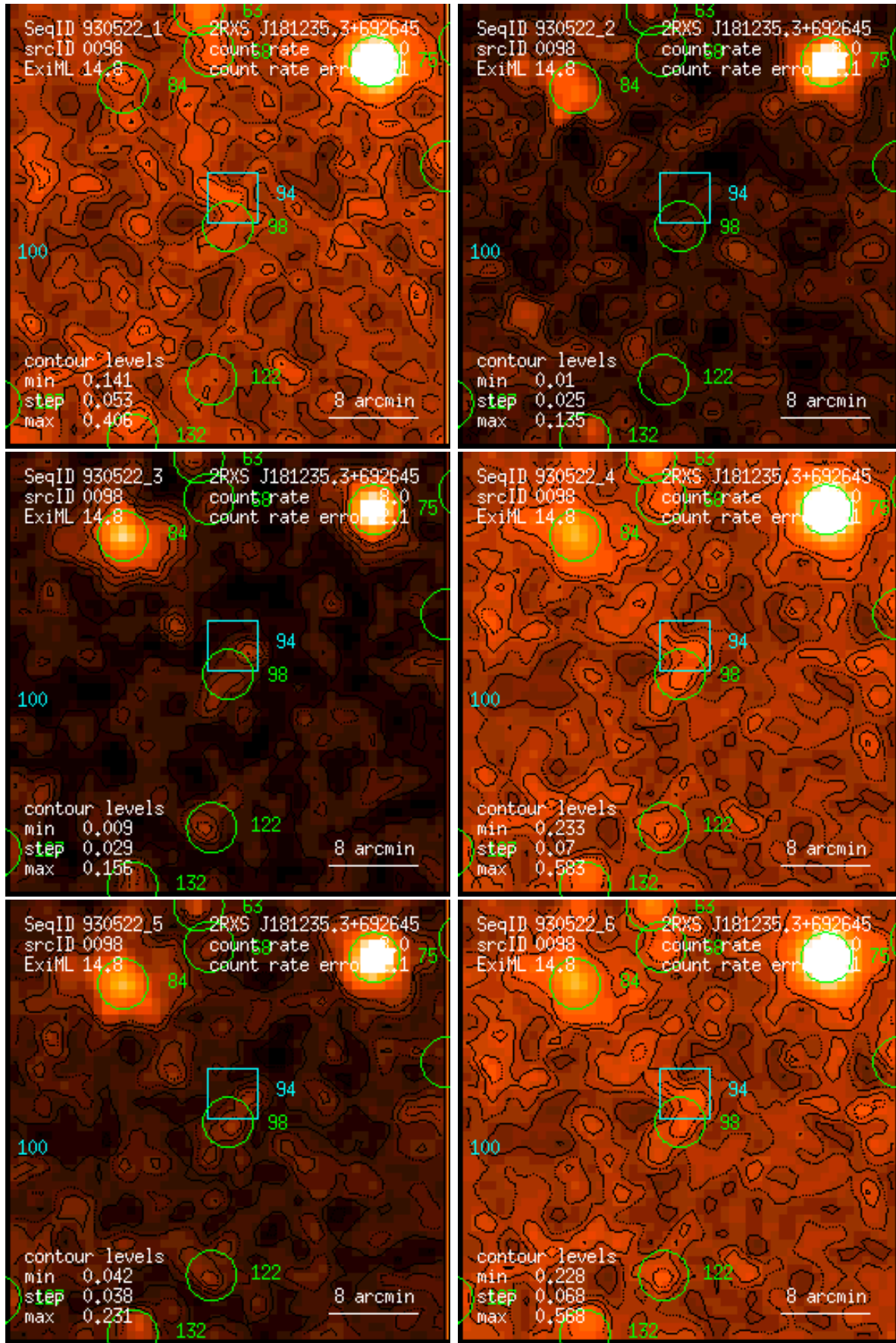
Figure 98: RASS 930522: detection 0098: band rate images, Gaussian filter: (1) PSPC channels 11 – 41, (2) 52 – 90, (3) 91 – 201, (4) 11 – 235, (5) 52 – 201, (6) 11 – 201. Broad band rates in counts/ks. Band rate contour levels in counts/ks/arcmin 2 .
