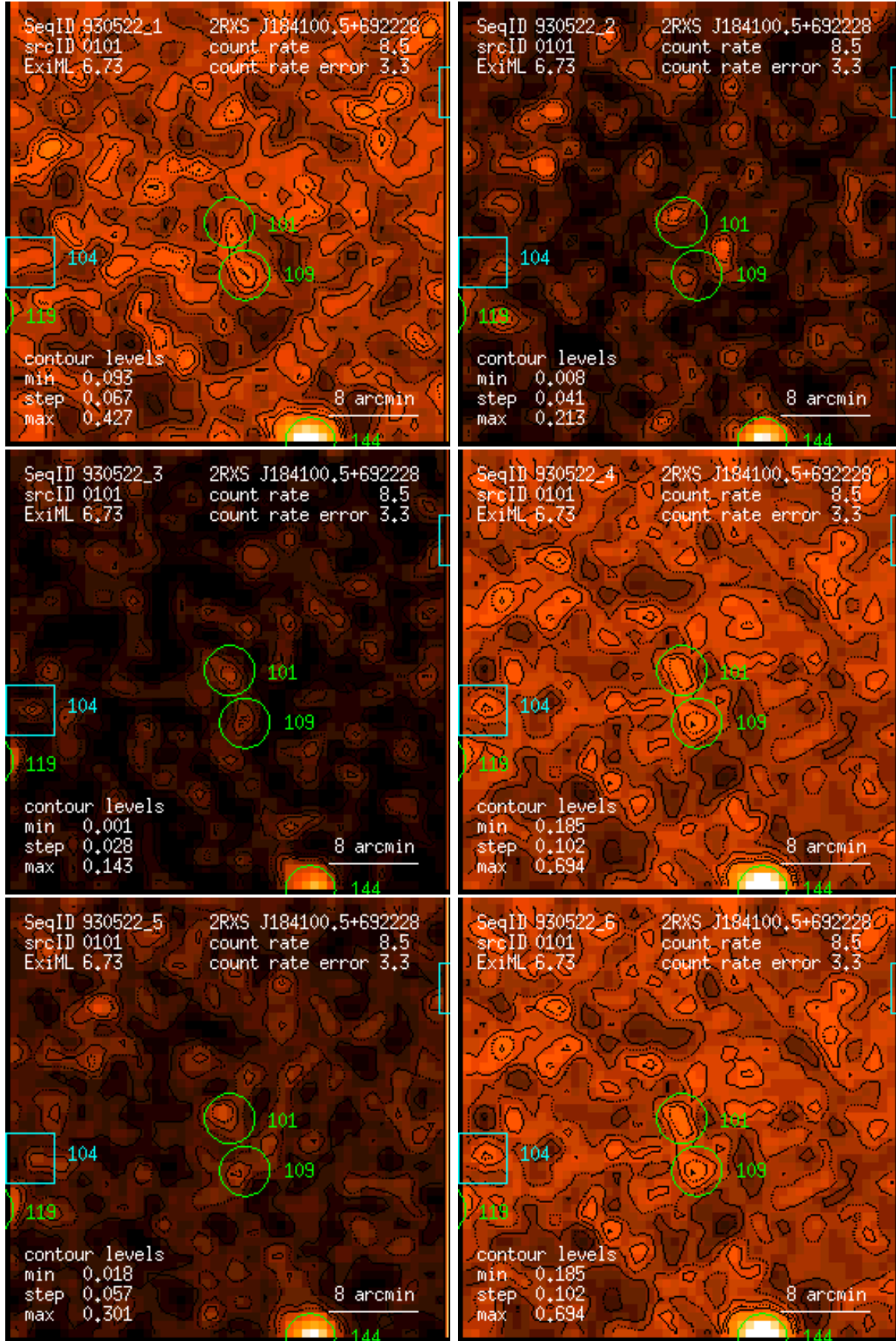
Figure 101: RASS 930522: detection 0101: band rate images, Gaussian filter: (1) PSPC channels 11 – 41, (2) 52 – 90, (3) 91 – 201, (4) 11 – 235, (5) 52 – 201, (6) 11 – 201. Broad band rates in counts/ks. Band rate contour levels in counts/ks/arcmin 2 .
